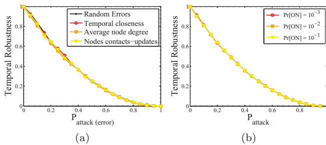
FIG. 4. (Color online) Temporal robustness as a function of removed (attacked) nodes percentage for Erdős-Rényi and Markov temporal network ( N = 100 , \tau = 150 ). Similar results are obtained (a) for different attacking strategies and fixed \text{Pr}[\text{ON}] = 10^{-3} ; and (b) for average node degree strategy and different probability of link appearance \text{Pr}[\text{ON}] .
