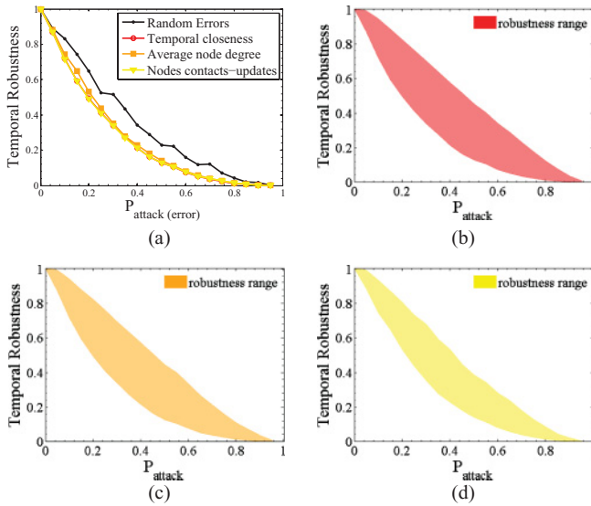
FIG. 10. (Color online) Temporal robustness and robustness range of INFOCOM temporal network ( \tau = 345600 ) as functions of removed (attacked) nodes percentage. (a) The temporal robustness is similar for different attacking strategies. The robustness range for (b) temporal closeness, (c) average node degree, and (d) nodes number of contacts-updates strategies.
