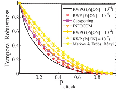
FIG. 12. (Color online) Temporal robustness of various temporal networks under unique attacking strategy (average node degree) as a function of attacked nodes percentage.
