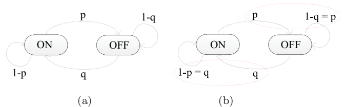
FIG. 2. (Color online) (a) Diagram for link appearance probabilities in Markov temporal model. (b) Erdős-Rényi temporal model. If p + q = 1 , one can notice that for each link the probability that the same is in the state ON is fixed and equal to q and does not depend on the previous state (ON or OFF). Similarly, for each link the probability that the same is in the state OFF is fixed and equal to p and does not depend on the previous state (ON or OFF). Consequently, it represents the Erdős-Rényi temporal model.
