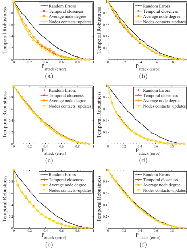
FIG. 7. (Color online) Temporal robustness of RWP and RWPG mobility models ( \tau = 3600 ) for different probability of link appearance \text{Pr}[\text{ON}] as a function of removed (attacked) nodes percentage. As \text{Pr}[\text{ON}] increases, temporal robustness decreases slowly and intelligent attack robustnesses are closer to the random error. (a) RWP: \text{Pr}[\text{ON}] = 10^{-4} ; (b) RWP: \text{Pr}[\text{ON}] = 10^{-3} ; (c) RWP: \text{Pr}[\text{ON}] = 10^{-1} ; (d) RWPG: \text{Pr}[\text{ON}] = 10^{-4} ; (e) RWPG: \text{Pr}[\text{ON}] = 10^{-3} ; and (f) RWPG: \text{Pr}[\text{ON}] = 10^{-1} .
