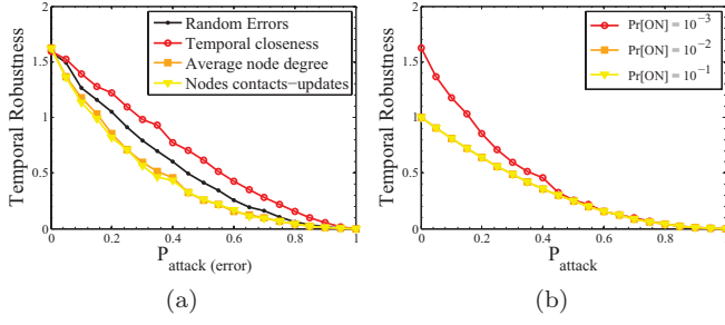
FIG. 3. (Color online) Temporal robustness as a function of removed (attacked) nodes percentage. The small \tau effect ( \tau = 20 ) in Erdős-Rényi temporal network. Variations and instability in temporal efficiency cause differences in temporal robustness. (a) For different attacking strategies and fixed \text{Pr}[\text{ON}] = 10^{-3} ; and (b) for average node degree strategy and different probability of link appearance \text{Pr}[\text{ON}] .
