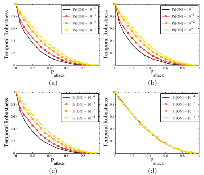
FIG. 6. (Color online) Temporal robustness as a function of removed (attacked) nodes percentage. RWPG mobility models ( \tau = 3600 ). (a) Temporal closeness, (b) average node degree, (c) nodes number of contacts-updates, and (d) random errors.
