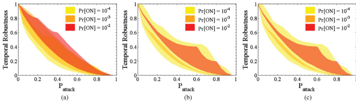
FIG. 9. (Color online) Robustness range of RWPG models ( \tau = 3600 ) for different attacking strategies: (a) temporal closeness, (b) average node degree, and (c) nodes number of contacts-updates as a function of removed (attacked) nodes percentage. As \text{Pr}[\text{ON}] decreases the robustness range area becomes wider.
