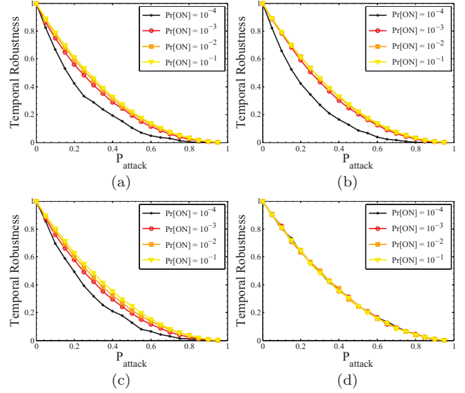
FIG. 5. (Color online) Temporal robustness as a function of removed (attacked) nodes percentage in RWP mobility models ( \tau = 3600 ). (a) Temporal closeness, (b) average node degree, (c) nodes number of contacts-updates, and (d) random errors.
