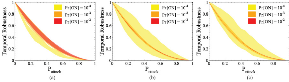
FIG. 8. (Color online) Robustness range of RWP models ( \tau = 3600 ) for different attacking strategies: (a) temporal closeness, (b) average node degree, and (c) nodes number of contacts-updates as a function of removed (attacked) nodes percentage. As \text{Pr}[\text{ON}] decreases, the robustness range area becomes wider.
