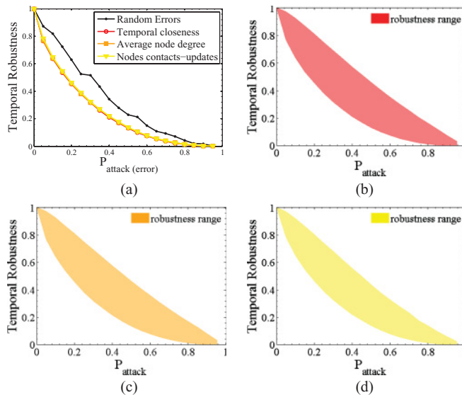
FIG. 11. (Color online) Temporal robustness and robustness range of Cabsplotting temporal network ( \tau = 86400 ) as functions of removed (attacked) nodes percentage. (a) The temporal robustness is similar for different attacking strategies. The robustness range for (b) temporal closeness, (c) average node degree, and (d) nodes number of contacts-updates strategies.
