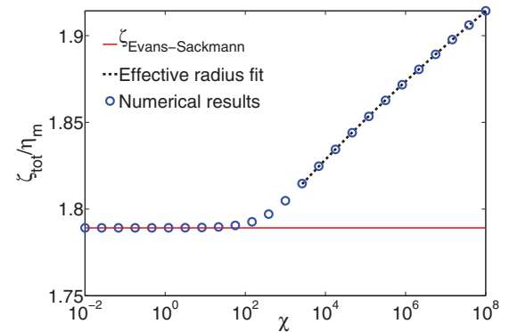
FIG. 8. (Color online) As \chi = \phi_b^2/\Gamma\eta_m is increased, the total drag on the protein \zeta_{\text{tot}} [Eq. (26)] increases only slowly, roughly as \ln\chi ; this is very different from the theory of Sec. II A, which predicts that the drag should be linearly proportional to \chi [Eq. (10)]. We can fit these results to an effective radius theory as suggested above, with R_{\text{eff}}/R = 1 + c_1 + c_2 \ln\chi with c_1 = -0.25 and c_2 = 0.045 . In this simulation, \epsilon = 10^{-3} , \beta = 10 , and \rho_{\max} = 100/\epsilon .
