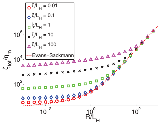
FIG. 13. (Color online) Increasing \chi increases the total drag \zeta_{\text{tot}} on the protein, but does not change the qualitative features from that shown in Fig. 12. For this figure, \chi = 10^5 . Only points with \beta < 10^3 are shown, for reasons of computation time.
