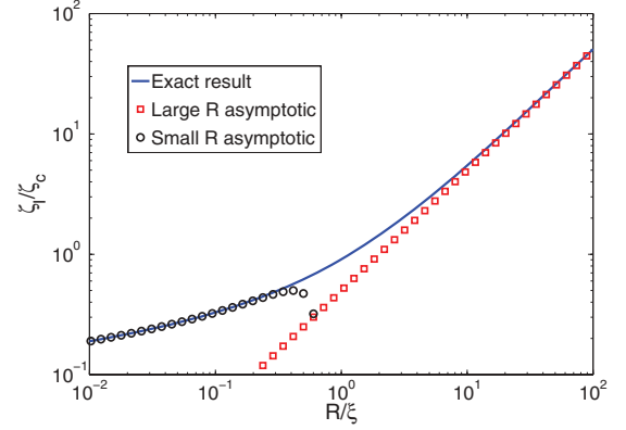
FIG. 3. (Color online) Drag from interaction with the external field [Eq. (10)] in the boundary condition model scales linearly with protein size for proteins with a radius much larger than the field's correlation length ( R \gg \xi ). However, in the limit R \ll \xi , \zeta_I \sim 1/\ln(R) [Eq. (11)].
