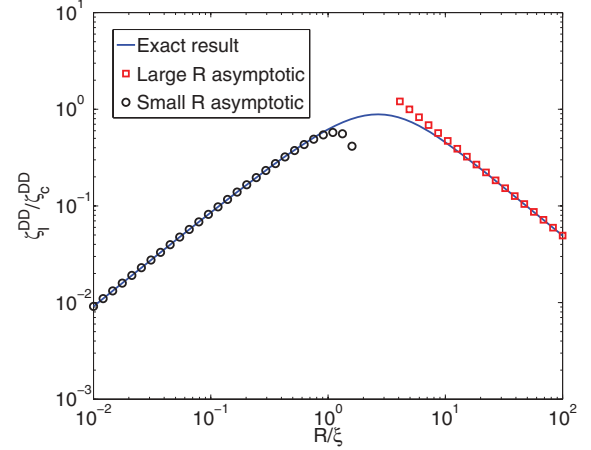
FIG. 4. (Color online) DD model [16], Eq. (16), predicts a drag coefficient \zeta_I^{\text{DD}} that scales linearly in protein size for R \ll \xi , but if we extend it naively into the limit R \gg \xi , \zeta_I^{\text{DD}} decreases with increasing protein size [Eq. (17)].
