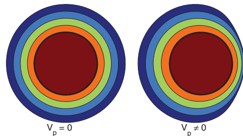
FIG. 2. (Color online) Illustration of the \phi(\mathbf{r}, t) profile. For the static protein (left), \phi(\mathbf{r}, t) = \phi_{(0)}(r) is given by Eq. (5). For a protein moving at constant rightward velocity (right), \phi(\mathbf{r}, t) = \phi_{(0)}(r) + V_0 \phi_{(1)}(r, \theta) . The contours shown are logarithmically spaced, i.e., \phi = \phi_b at the thick contour ( r = R ), and \phi = 0.1\phi_b at the next contour out.
