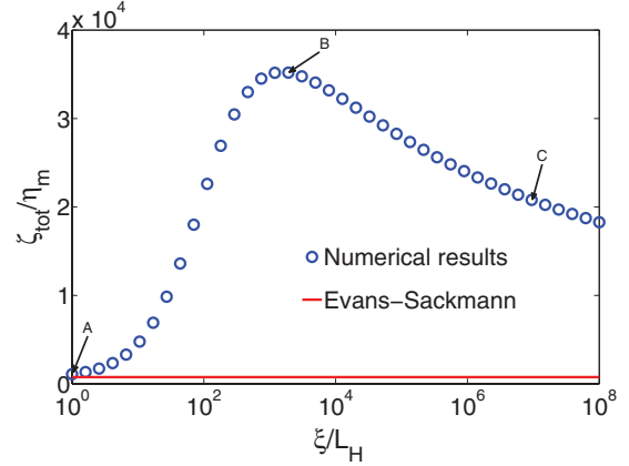
FIG. 14. (Color online) Total drag on the protein \zeta_{\text{tot}} [Eq. (26)] can be nonmonotonic in \xi , the size of the distortion of the \phi field. The velocity field of the points marked A, B, and C are shown in Fig. 15. For this simulation, \epsilon = 10 and \chi = 10^5 , and we set \rho_{\text{max}} = \max(100, 100/\beta) , where \beta = R/\xi ; this result is insensitive to increases in \rho_{\text{max}} and refinements of the mesh.
