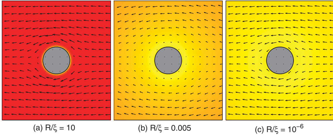
FIG. 15. (Color online) Lipid flow fields near the protein are superimposed over the distortion in the order parameter, \phi_{(0)}(\mathbf{r}) , which is shown as a color map, ranging from light ( \phi = \phi_b ) to dark ( \phi = 0 ). Velocities are plotted relative to the protein's velocity. In the leftmost image (a), the distortion is small, and does not strongly affect the velocities. In the center image (b), the distortion is large, extending far beyond the region shown, but still shows noticeable gradients near the protein. In this limit, lipids are significantly correlated to the protein over a larger range than shown in (a). In (c), the distortion is yet larger, and the gradient near the protein has decreased; lipids near the protein are not as entrained as in (b). The velocities have the same scale for (a), (b), and (c).
