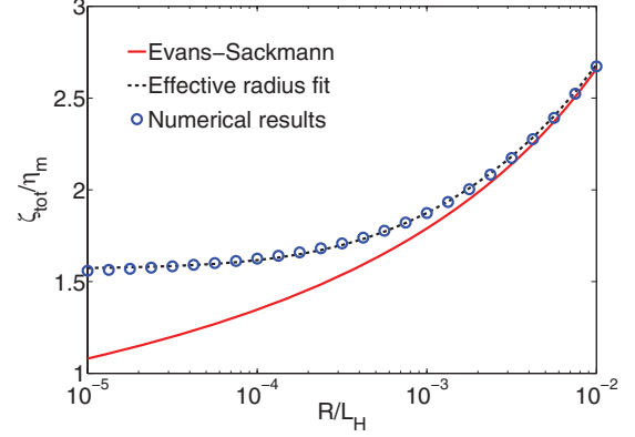
FIG. 10. (Color online) As the radius of the particle is increased, the additional drag from the order interaction becomes negligible and \zeta_{\text{tot}} [Eq. (26)] approaches \zeta_{\text{Evans-Sackmann}} . In this figure, we vary R while keeping \xi and L_H fixed; we thus vary \beta and set \epsilon = 10^{-4}\beta , so that \epsilon \ll 1 for the entire range of \epsilon studied ( \beta ranges from 0.1 to 100). \chi = 10^6 for this figure. This is well fit to an effective radius of R_{\text{eff}}/R = 1 + c/\beta with c = 3.73 .
