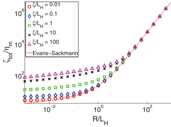
FIG. 12. (Color online) As the radius of the object increases, the additional drag from the order parameter interaction becomes negligible and the total drag \zeta_{\text{tot}} [Eq. (26)] approaches the Evans-Sackmann result as R \gg \xi, L_H . Drag is shown as a function of R/L_H = \epsilon , with L_H and \xi held fixed. For this figure, \chi = 10^3 . Only points with \beta < 10^3 are shown, for reasons of computation time.
