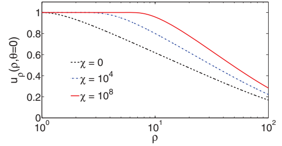
FIG. 7. (Color online) As \chi = \phi_b^2/\Gamma\eta_m is increased, the lipids near the protein are increasingly correlated to the protein velocity, and the radial velocity profile u_\rho is constant over the effective radius of the protein, which increases weakly with increasing \chi . For this figure, \beta = 1 , \epsilon = 10^{-2} , and \rho_{\max} = 100/\epsilon (the entire domain is not shown in this figure).
