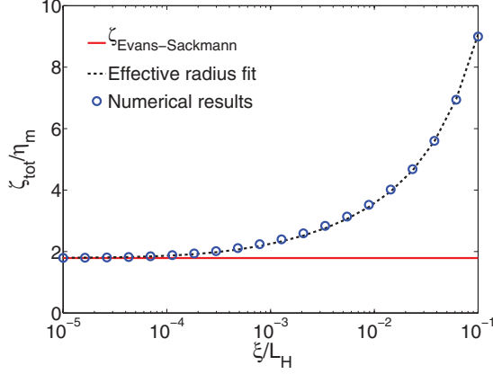
FIG. 9. (Color online) If we vary the correlation length of \phi , \xi , while holding the radius R and the hydrodynamic length scale L_H fixed (corresponding to varying \beta while holding \epsilon fixed), we see that smaller drag layers lead to smaller total drag \zeta_{\text{tot}} [Eq. (26)] on the particle. This should be contrasted with the result in the absence of hydrodynamics, Eq. (10), in which thinner layers lead to larger gradients and thus larger drags. \epsilon = 10^{-3} and \chi = 10^6 for the data in this figure. This is well fit to an effective radius of R_{\text{eff}}/R = 1 + c/\beta with c = 3.22 .
