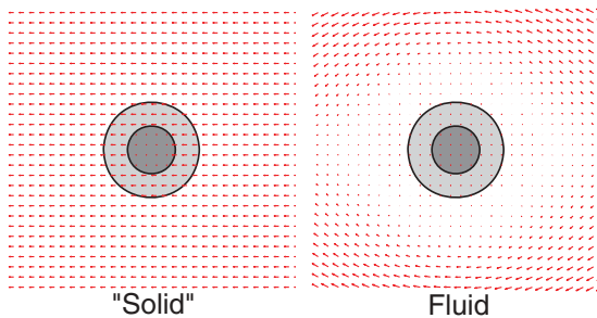
FIG. 5. (Color online) Lipid velocities plotted in the frame moving with the protein. The dark central circle is the protein, and the lighter circle the region with \phi(\mathbf{r}) significantly different from 0. The models of Sec. II make the assumption that the lipids are at rest relative to the protein, i.e., that they have velocity -\mathbf{V}_p in the protein's rest frame; this is illustrated in the left panel. In a fluid membrane, the lipid velocity will be entrained by the protein motion (right). The distortion of the profile \phi(\mathbf{r}) will be significantly reduced in this case, compared to that of Sec. II.
