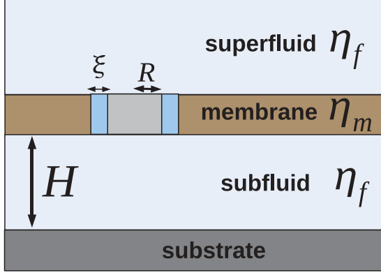
FIG. 6. (Color online) Illustration of protein of radius R diffusing in membrane a height H above a substrate, surrounded by fluid with viscosity \eta_f . We have also indicated the distorted region near the membrane, with characteristic size \xi .
