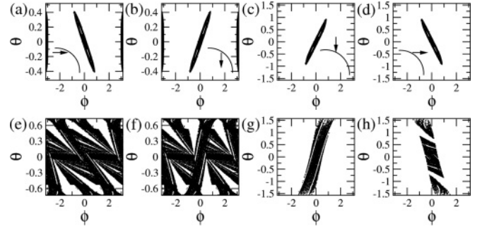
FIG. 7. The generalized PSOSs constructed by considering the (a, e) incident ray inside, (b, f) emerging ray inside, (c, g) incident ray outside, and (d, h) emerging ray outside cavities, which is schematically represented in each inset in the upper row. We choose n = 2.0 (the upper row) and n = 1.5 (the lower row) with D = 0.1 and R_R = R_L = 1.0 .
