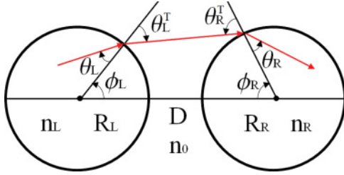
FIG. 2. (Color online) Schematic picture of the coupled two disks. The red (gray) straight lines with arrows represent a typical trajectory of a ray transmitted from the left (L) to the right (R) disk. Note that in the left disk \phi_L and \theta_L increases in the counterclockwise direction, while in the right disk the opposite is true. For example, in this figure, \phi_L , \phi_R , \theta_R , and \theta_R^T are positive, and \theta_L and \theta_L^T are negative. R_L and R_R is the radius of the left and the right disk, respectively, and D is the distance between two disks. n_L , n_R , and n_0 are the indices of refraction of the left disk, the right disk, and the outside, respectively.
