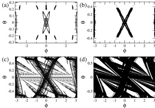
FIG. 6. The PSOSs of the asymmetric TDM of R_R = 1.1 R_L obtained in the left disk. (a) n = 3.3 , (b) n = 2.0 , (c) n = 1.8 , and (d) n = 1.5 with D = 0.1 .
