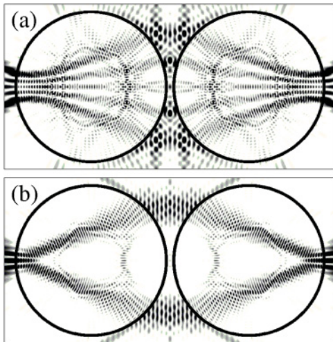
FIG. 4. Patterns of resonant modes obtained from wave calculation when (a) n = 2.0 and (b) n = 1.8 , which are directly associated with the islands of Fig. 3(b) and 3(c), respectively.
