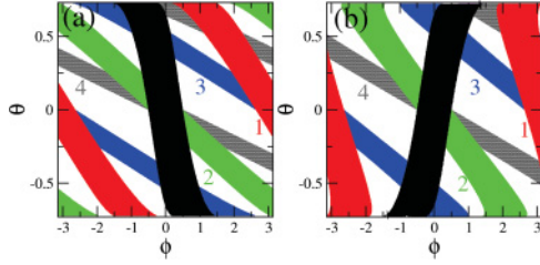
FIG. 5. (Color online) The first (red/gray), second (green/light gray), third (blue/dark gray), and fourth (silver/scratched gray) iterated sets according to Eq. (9) starting from (a) the outgoing (black) and (b) the incoming area (black).
