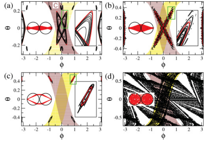
FIG. 3. (Color online) The PSOs of the two-disk map (TDM) for (a) n = 3.3 , (b) n = 2.0 , (c) n = 1.8 , and (d) n = 1.5 with D = 0.1 and R_R = R_L = 1.0 . The right insets of (a)–(c) represent the corresponding enlarged PSOs of the part of the islands designated by the green boxes. The left insets represent the trajectories in real space corresponding to (a)–(c) the torus denoted as the thick red curve in the islands and (d) the chaotic quasiattractor. The outgoing (also called region C) and the incoming area are represented as brown (dark gray) and yellow (light gray) area, respectively. They are symmetric over \phi = 0 and \theta = 0 due to the symmetric geometry shown in Fig. 2.
