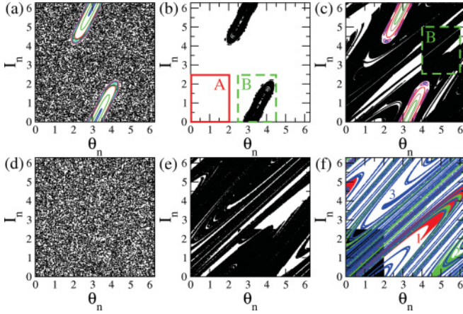
FIG. 1. (Color online) PSOSs of standard mapping for (a) K = 4.0 and (d) K = 9.0 . Different color sets represent those from different initial points. The PSOSs of the combined standard-linear map; (b, c) for K = 4.0 and (e, f) for K = 9.0 . The region A is denoted as the red solid box in (b). The region B, denoted as the dashed green box, is chosen as (b, e) (\alpha, \beta) = (2.5, 0.0) and (c) (\alpha, \beta) = (4.0, 2.5) . (f) Forward iterated sets starting from the region A using only the standard map. Red (gray), green (light gray), and blue (dark gray) sets represent the first, second, and third iterated sets, respectively.
