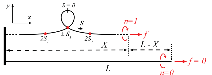
FIG. 12. (Color online) Properties of the homoclinic planar elastica, configuration \bar{b} in Fig. 10.
