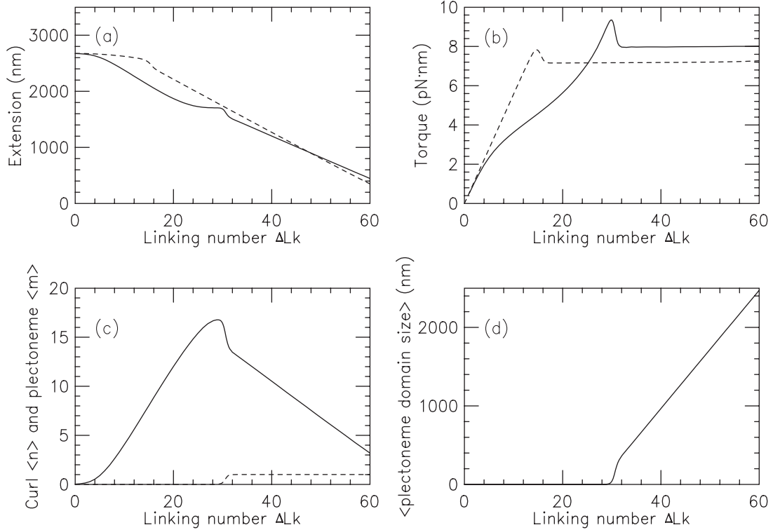
FIG. 8. Behavior of supercoiled DNA in the presence of curl-binding proteins. Calculations are shown for f = 0.5 pN, 150 mM salt, and \beta\mu = 10 . The presence of the curl-binding proteins stabilizes the curls and drives formation of many curls at the buckling transition. Extension as a function of \Delta Lk is shown as the solid curve in (a); torque is shown as the solid curve in (b); dashed curves indicate results without curl-binding proteins from Fig. 5. Curl ( \langle n \rangle , solid) and plectoneme ( \langle m \rangle , dashed) numbers are shown in (c) for the curl-binding protein case; the corresponding interwound length per plectoneme ( \langle L_p/m \rangle ) is shown in (d).
