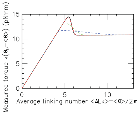
FIG. 9. (Color online) Measured torque for 2.2-kb DNA in 150 mM salt buffer under 1-pN force, for spring constants k = 1, 0.1 , and 0.01 k_B T/\text{rad}^2 (dashed uppermost red, middle green, and bottom blue curves, respectively). Torque overshoot is smoothed out as k is decreased, but small values of k are needed to completely eliminate it. The k = 1 curve is indistinguishable from the “true” torque [solid black, same as 1-pN curve in Fig. 3(b)].
