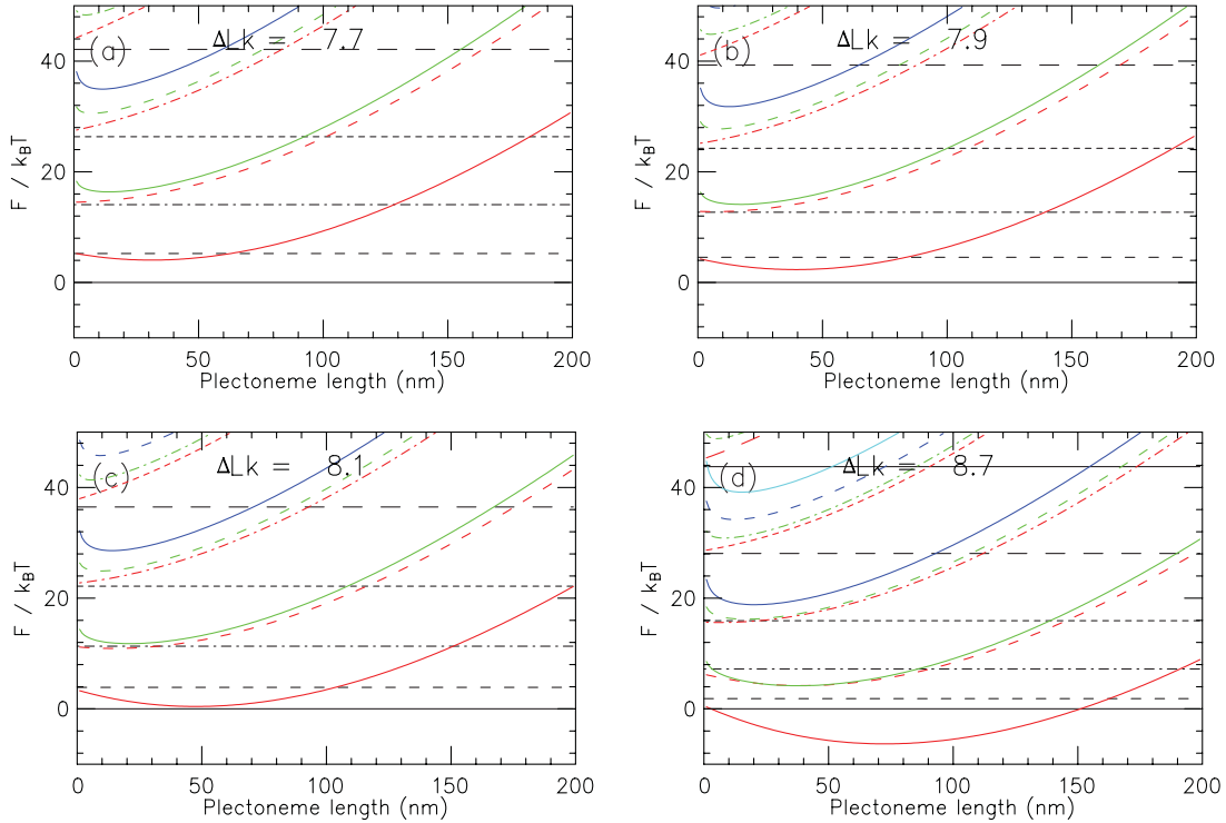
FIG. 2. (Color online) Free energies of states with different (n, m) and L_p near buckling transition for 2.2-kb molecule in 150 mM \text{Na}^+ buffer subject to 2-pN force. Free energies are measured relative to that of the n = 0, m = 0 state. Horizontal black lines indicate straight DNA with different numbers of chiral curls and no plectonemic domains ( m = 0 ): solid, n = 0 ; dashed, n = 1 ; dot-dashed, n = 2 ; short dashed, n = 3 ; long dashed, n = 4 . Curves indicate free energy as a function of length of interwound plectonemic region for states with successively larger numbers of plectonemic regions: The line dash style indicates the number of curls in that state, following the same labeling as the straight-curl states. Plectonemic states with m = 1, 2, 3 , and 4 for each value of n (each dash type) have free energies which increase with m for each value of plectoneme length ( m = 1, 2, 3 , and 4 are shown in red, green, blue, and cyan, respectively). Parts (a), (b), (c), and (d) show the free energies for successively larger linking numbers passing through the buckling transition. The uppermost solid line in (d) shows the (5, 0) state.
