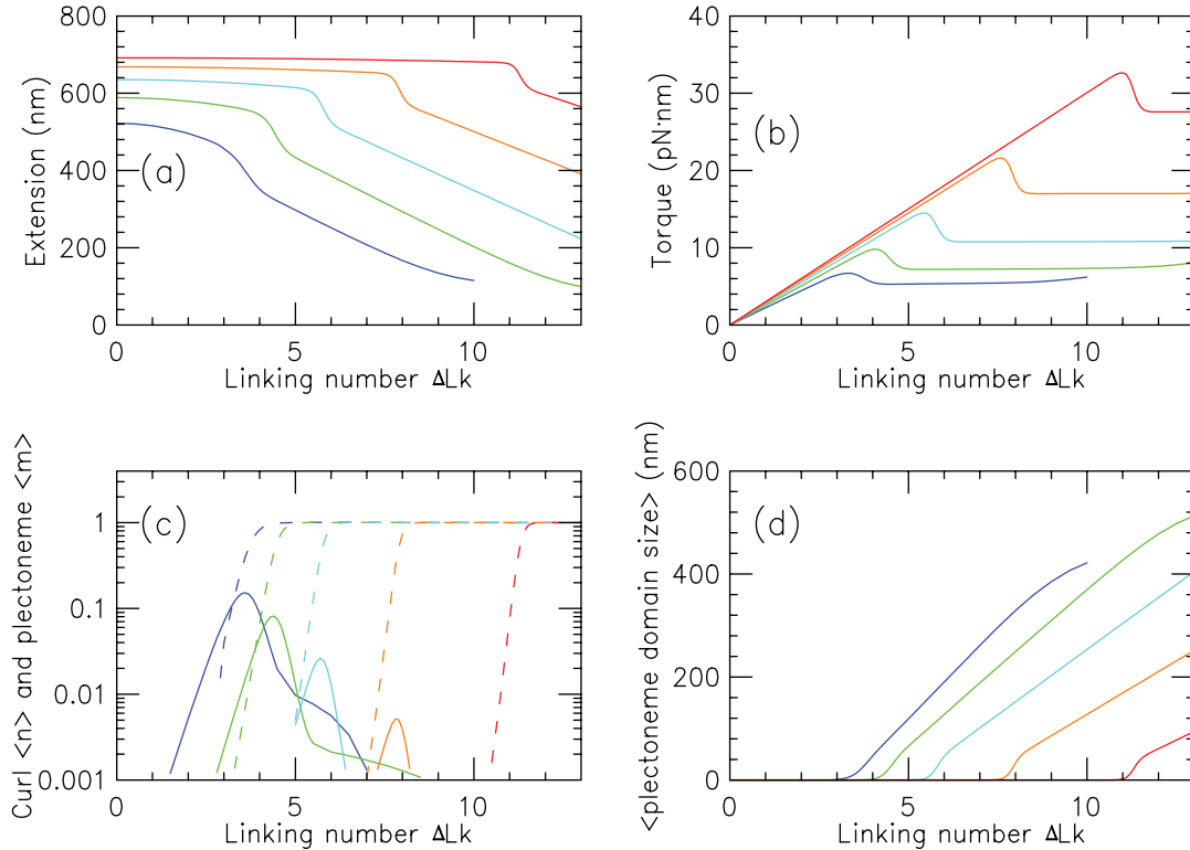
FIG. 3. (Color online) Properties of stretched twisted DNA as a function of linking number, for a 2.2-kb molecule in 150 mM Na + buffer, for forces of 0.25 (blue), 0.5 (green), 1 (cyan) 2 (orange), and 4 pN (red). (a) Extension versus linking number (curves show results for successively higher forces from bottom to top). (b) Torque versus linking number (curves show results for successively higher forces from bottom to top). (c) Average number of plectonemic ( \langle m \rangle , dashed) and curl ( \langle n \rangle , solid) regions (solid curves show \langle n \rangle values for successively higher forces from left to right for 0.25 to 2 pN, with the 4-pN results too small to appear on this plot; dashed curves show \langle m \rangle values for successively higher forces from left to right). (d) Mean plectoneme domain size ( \langle L_p/m \rangle ) for states containing interwound plectonemic regions (curves show results for successively higher forces from left to right).
