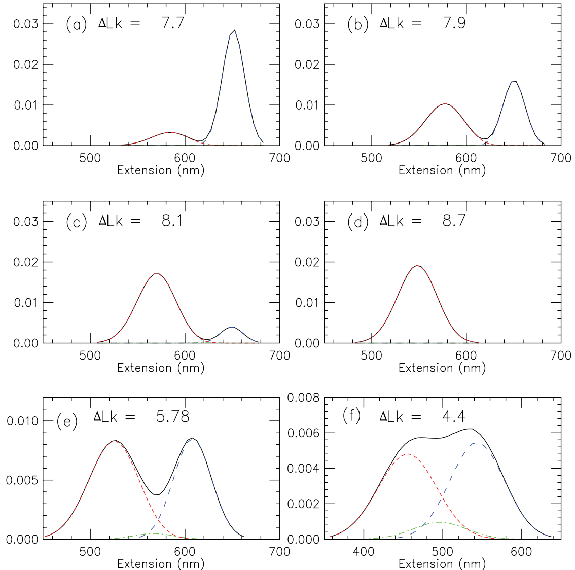
FIG. 4. (Color online) (a)–(d) Extension distribution near buckling transition for 2.2-kb DNA, 150 mM Na + buffer, corresponding to curves shown in Fig. 2. ( f = 2 pN, \Delta Lk as indicated in panels). Contributions from extended DNA without plectonemic or curl domains (blue, long dashed, peak to right), states with plectonemically supercoiled DNA (red short dashed, peak to left), and states with chiral curls and no plectonemes (green dot-dashed, low peak in middle) and their sum (black solid) are shown. As the buckling transition is approached by gradually increasing linking number, the extension distribution changes from being dominated by the extended state to being dominated by plectonemes; a double-peak distribution is obtained at the buckling point. Near the buckling point only a small number of chiral curls appear. (e) and (f) Extension distribution at buckling transition for 2.2-kb DNA, 150 mM Na + buffer, \Delta Lk as indicated in panels, for (e) f = 1 pN and (f) f = 0.5 pN. For these lower forces the extension histogram loses its bimodal shape, and the contribution from curl fluctuations becomes larger (dot-dashed line, green).
