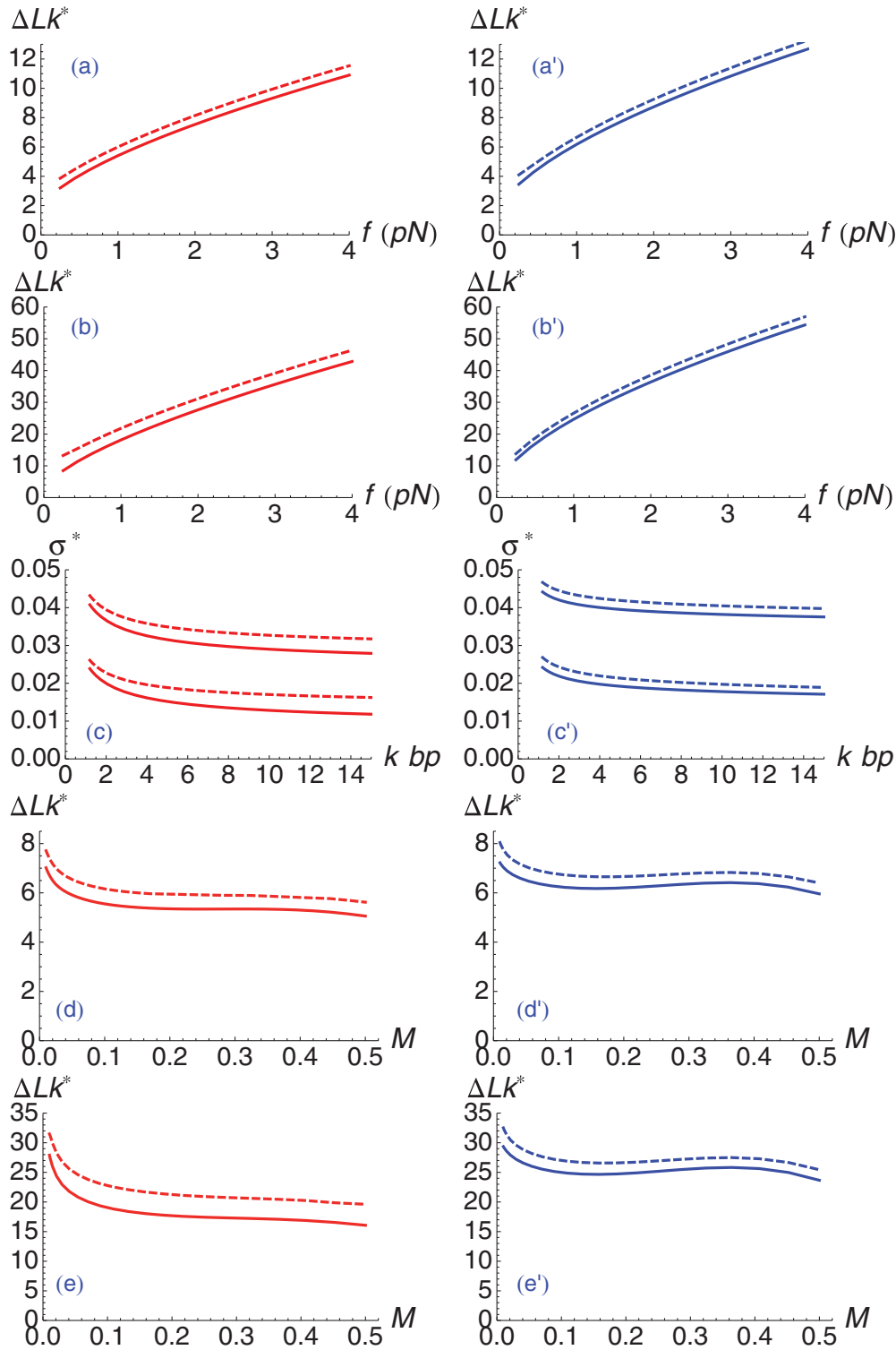
FIG. 7. (Color online) Dependence of one-plectoneme transition point \Delta Lk_{m=1}^* (left column) and one-curl transition point \Delta Lk_{n=1}^* (right column) with force, salt, and length. For each panel in left column, solid curves show approximate formula (22); in right column to (24). Dashed curves in left column are numerical solutions of \beta F(0,0,0) = \beta F(0,1,L_p) obtained by minimizing the complete free energy (12); in right column corresponding solutions for \beta F(0,0,0) = \beta F(0,1,L_p) are shown. The different panels show results for: (a) (a') 2.2 kbp and 150 mM, as a function of force (pN); (b) (b') 10 kbp and 150 mM, as a function of force (pN); (c) (c') supercoiling density \sigma \equiv 10.5 \Delta Lk/(nbp) for 150 mM and 0.5 pN (lower curves), 2 pN (upper curves), as a function of DNA length (kbp); (d) (d') 2.2 kbp and 1 pN, as a function of univalent salt concentration (M); (e) (e') 10 kbp and 1 pN, as a function of univalent salt concentration (M).
