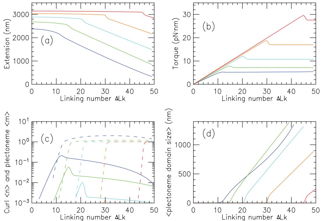
FIG. 5. (Color online) Properties of stretched twisted DNA as a function of linking number, for a 10-kb molecule in 150 mM \text{Na}^+ buffer, for forces of 0.25 (blue), 0.5 (green), 1 (cyan), 2 (orange), and 4 pN (red). (a) Extension versus linking number (curves show successively higher forces from left to right). (b) Torque versus linking number (curves show successively higher forces from bottom to top). (c) Average numbers of plectonemic regions ( \langle m \rangle , dashed; curves show successively higher forces, from left to right) and curls ( \langle n \rangle , solid; curves show successively higher forces from left to right). (d) Mean plectoneme domain size ( \langle L_p/m \rangle ) for states containing interwound plectonemic regions (curves with successively higher forces have starting points at zero domain size that are located at successively larger linking number values).
