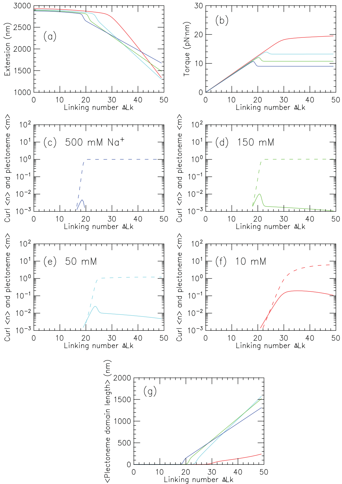
FIG. 6. (Color online) Salt dependence of properties of a stretched twisted DNA, as a function of linking number, for a 10-kb molecule for Na^+ concentrations of 10 mM (red), 50 mM (cyan), 150 mM (green) and 500 mM (blue), for a force of 1 pN. (a) Extension versus linking number; curves at \Delta Lk = 20 run from top to bottom with increasing salt concentration. (b) Torque versus linking number; curves show results for successively higher salt concentrations from top to bottom. (c)–(f) Average number of plectonemic (dashed) and curl (solid) regions for (c) 500 mM, (d) 150 mM, (e) 50 mM, and (f) 10 mM. (g) Mean plectoneme domain size ( \langle L_p/m \rangle ) for states containing interwound plectonemic regions (curves with successively higher salt have starting points at zero domain size that are located at successively smaller linking number values).
