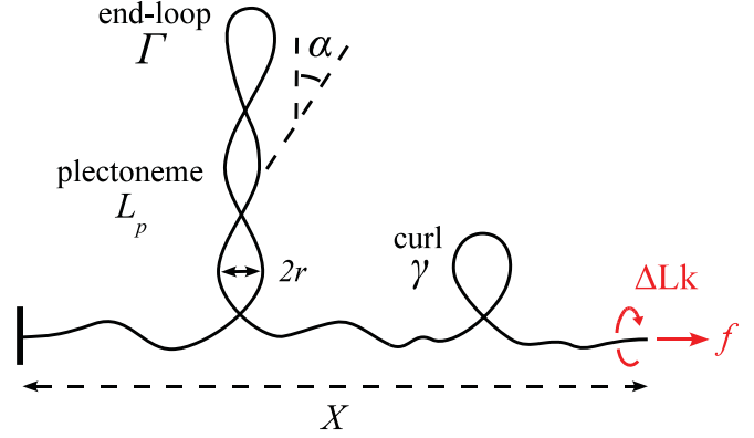
FIG. 1. (Color online) Sketch of a conformation of an extended DNA with a plectonemic domain, and a chiral curl.
