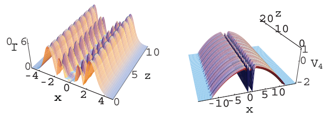
FIG. 4. (Color online) Fourth-order ( n = 4 ) solitary wave (16) generated by the dark seed wave form (7b). The corresponding parameters are given in the text.
