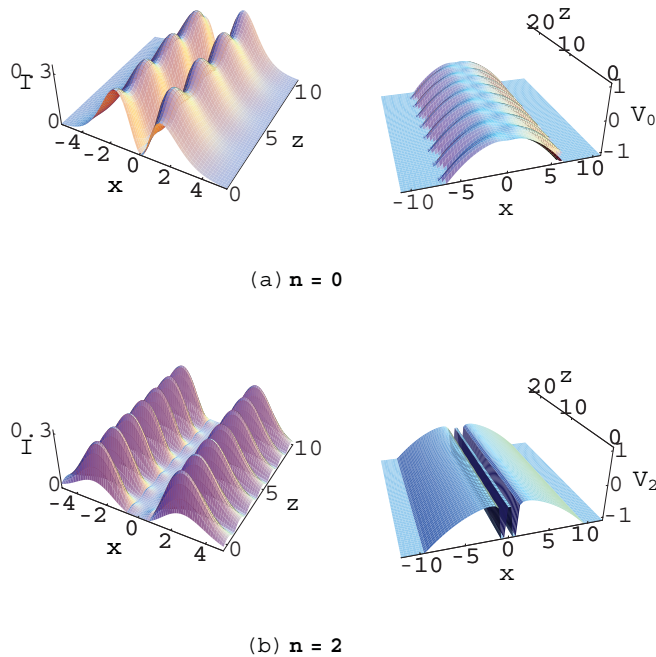
FIG. 2. (Color online) Plots of the breathing solitary waves (16) generated by the dark seed (7b) (the corresponding parameters are given in the text). The setup here and in Figs. 3 and 4 below is the same as in Figs. 1(a) and 1(b).
