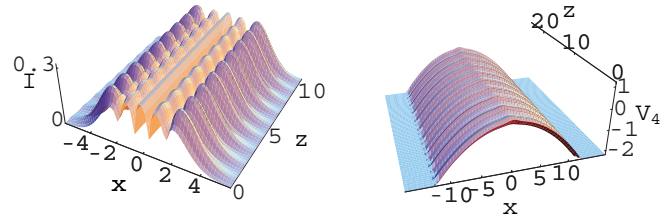
FIG. 3. (Color online) Fourth-order bright solitary wave. The corresponding parameters are given in the text.
