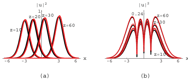
FIG. 5. (Color online) Comparison of the analytical solution with the numerical simulations at different propagation distances. The black solid line is the analytical solution given by Eq. (16) and the dashed red line is the result of the simulation of Eq. (1). (a) The setup is the same as in Fig. 1(a), the propagation distance being z = 10, 20, 30, 60 from left to right. (b) The same as in (a), except for n = 3 ; the propagation distance is z = 10, 30, 60 from bottom to top.
