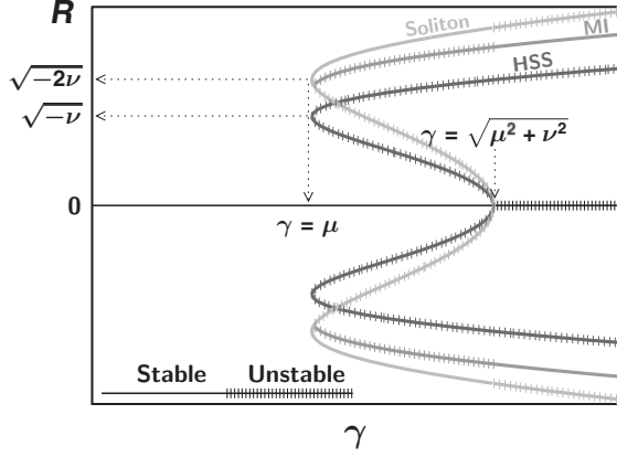
FIG. 2. Bifurcation diagram of the parametrically driven of the solitons [Eqs. (9)] of the parametrically driven damped nonlinear Schrödinger equation. In this diagram, we assume that we are close enough to the curve \gamma(v) = \sqrt{\mu^2 + \nu^2} , so the periodic or chaotic oscillation of the stable soliton is avoided [30]. Discussion about the stability of the homogeneous steady state (HSS) can be found in Ref. [20]. MI refers to the maximum amplitude of the standing waves ( \psi^{sw} ).
