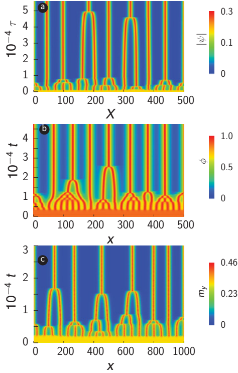
FIG. 1. (Color online) Cascade of coalescence processes observed numerically in (a) the parametrically driven damped nonlinear Schrödinger equation ( \mu = 0.050 , \gamma = 0.053 , \nu = -0.03 ), (b) a parametrically vertically driven pendula chain ( \mu = 0.100 , \gamma = 0.212 , \nu = -0.030 ), and (c) easy-plane ferromagnetic spin chain exposed to a periodic external field ( H = 0.200 , h = 0.044 , \beta = 4.800 , \alpha = 0.020 , \nu = -0.030 ).
