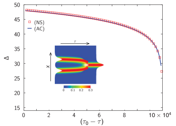
FIG. 4. (Color online) Temporal evolution of soliton separation distance \Delta(\tau) for \mu = 0.05 , \gamma = 0.054 , and \nu = -0.04 . Red squares stand for the numerical simulation of Eq. (1) and the continuous curve is deduced from formula (20). The inset gives the spatiotemporal diagram of the amplitude of \psi .
