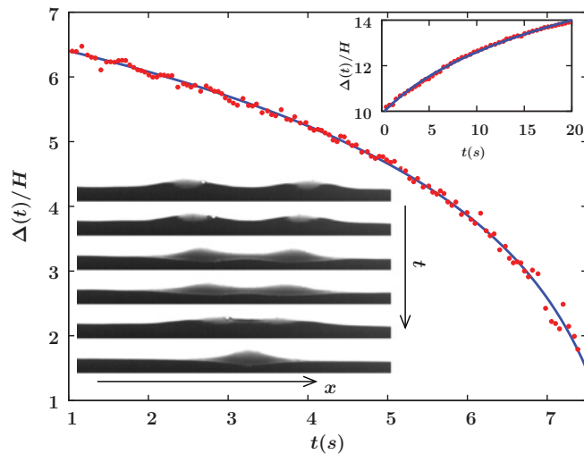
FIG. 5. (Color online) Temporal evolution of separation distance of a pair of in-phase and out-of-phase [inset (b)] solitons in a vertically driven rectangular water container (red filled circles). The fit \Delta(t) = a \ln[-b(t - t_0)] (blue solid line) of the experimental data, motivated by formula (20) gives a/H = 2.20 \pm 0.04 , b = 2.7 \pm 0.1 \text{ s}^{-1} , and t_0 = 8.20 \pm 0.04 \text{ s} for the in-phase solitons and a/H = 3.00 \pm 0.04 , b = 4.0 \pm 0.2 \text{ s}^{-1} , and t_0 = 6.7 \pm 0.1 \text{ s} for the out-of-phase solitons. Inset (b) gives snapshots of the experiment of in-phase soliton interaction at some arbitrary given times.
