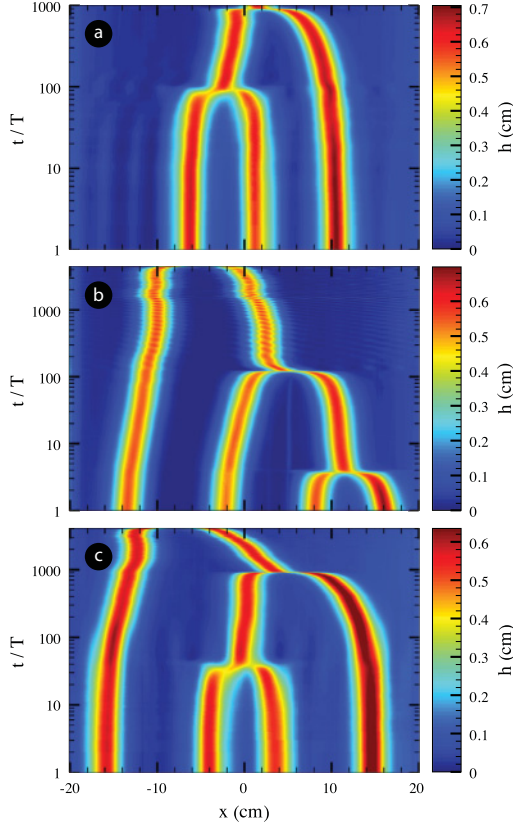
FIG. 6. (Color online) Multisoliton state evolution on the free surface of a 50 \times 1.54 \text{ cm}^2 rectangular basin filled with water (2 cm depth). The figures show the spatiotemporal diagrams (logarithmic time scale) for three different realizations, unveiling coalescence cascade processes. The images are taken stroboscopically. The forcing frequency is \nu = 14 \text{ Hz} and the amplitudes are (a) \Gamma = 0.202 (three solitons) and (b) and (c) \Gamma = 0.201 (four solitons).
