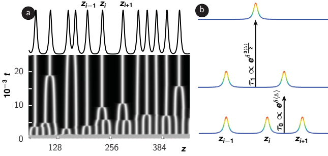
FIG. 7. (Color online) (a) Amplitude spatiotemporal density plot of numerical solution of Eq. (1) for \mu = 0.05 , \gamma = 0.053 , and \nu = -0.03 . The black solid line represents the profile at a given time. (b) Geometrical picture of the three interacting solitons.
