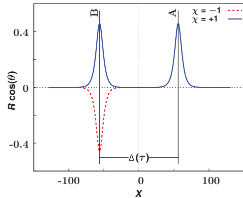
FIG. 3. (Color online) Illustration of a state of a pair of interacting dissipative solitons. The aim of the theoretical study of Sec. III A is the determination of the effective phase and the instantaneous velocity ( \dot{\Delta} ) of solitons.
