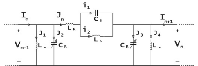
FIG. 2. The unit-cell circuit of the SRR-CPW model.
