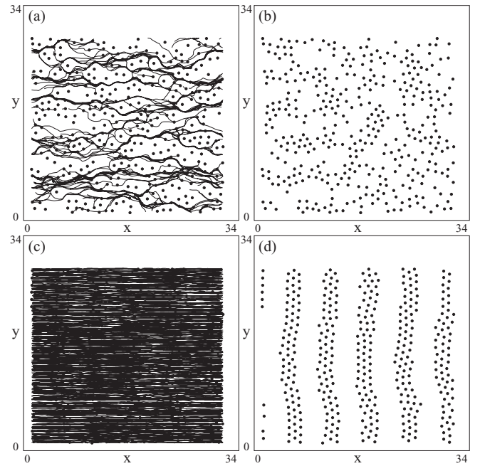
FIG. 5. The particle positions (black dots) and particle trajectories (black lines) for the system in Figs. 2(c) and 2(d) for pulse driving in the x direction. The particle trajectories are traced over equal times in panels (a) and (c). (a) At F_D^x = 0.125 , fluctuating plastic flow occurs in which channels of moving particles intertwine and mix while other particles remain pinned. (b) The particle positions only for the system in (a) indicate that the stripe structures are completely disordered. (c) At F_D^x = 0.23 , above the peak in d\langle V_x \rangle/dF_D^x shown in Fig. 2(d), all the particles are moving in an ordered transverse moving stripe phase. (d) A plot of only the particle positions from (c) shows the ordered stripes.
