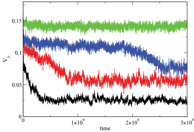
FIG. 4. (Color online) The velocity V_y in the y direction averaged over every 200 simulation time steps vs time in simulation time steps for pulse drives of F_D^y = 0.11, 0.125, 0.15, and 0.17 , from bottom to top. In the lower three curves, which fall in the strongly fluctuating plastic flow regime, the transition from a higher to a lower velocity occurs when the ordered stripe structure breaks apart, such as when the structure seen in Fig. 3(f) turns into a fragmented structure of the type shown in Fig. 3(d). The upper curve is at a drive above the transition to the moving ordered stripe regime.
