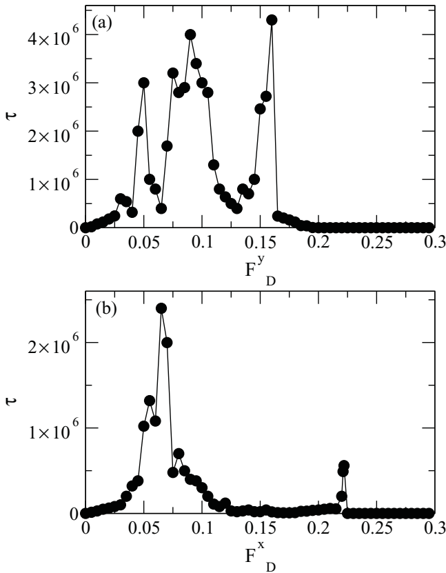
FIG. 6. The time \tau in simulation time steps required for the system to reach a steady state velocity after an applied pulse drive for the system in Fig. 2. (a) \tau vs F_D^y for driving in the y direction. The first peak at F_D^y = 0.04 corresponds to the depinning transition, the second peak centered at F_D^y = 0.1 appears at the transition from the filamentary flow illustrated in Figs. 3(a) and 3(b) to the fluctuating flow state shown in Figs. 3(c) and 3(d), and the third peak at F_D^y = 0.165 is associated with the transition to a moving ordered stripe state. (b) \tau vs F_D^x for driving in the x direction.
