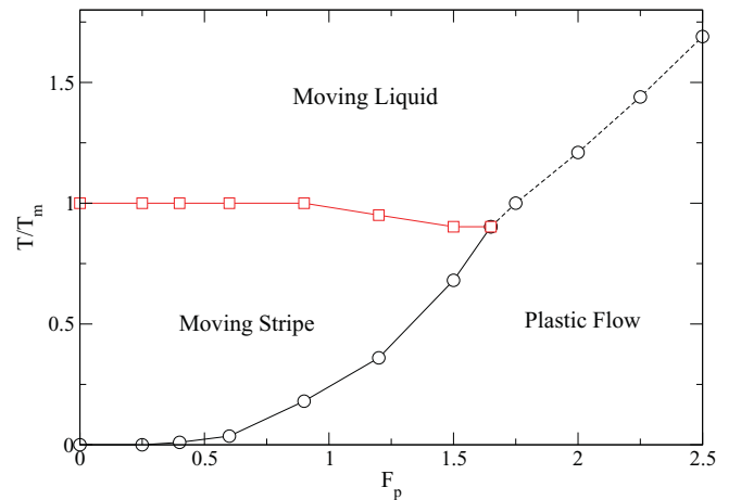
FIG. 21. (Color online) Phase diagram of T/T_m vs F_p for a system with \rho_p = 0.38 , R_p = 0.2 , and a y -direction drive of F_D^y = 0.22 . Here T_m is the melting temperature for the system without quenched disorder. The lower solid line separates the plastic flow phase from the moving stripe phase and the upper solid line separates the moving stripe phase from the moving liquid phase. The dashed line separates the plastic flow phase from the moving liquid phase. The phase diagram shows that for intermediate pinning strength, increasing the temperature can produce a transition from a disordered plastic flow phase into an ordered moving stripe phase.
