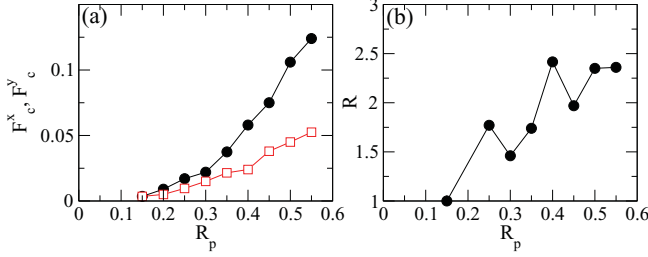
FIG. 16. (Color online) (a) F_c^x (filled circles) and F_c^y (open squares) vs R_p for a system with F_p = 0.225 and \rho_p = 0.38 . (b) The ratio R = F_c^x / F_c^y vs R_p showing that the anisotropy increases with increasing R_p and saturates at high R_p .
