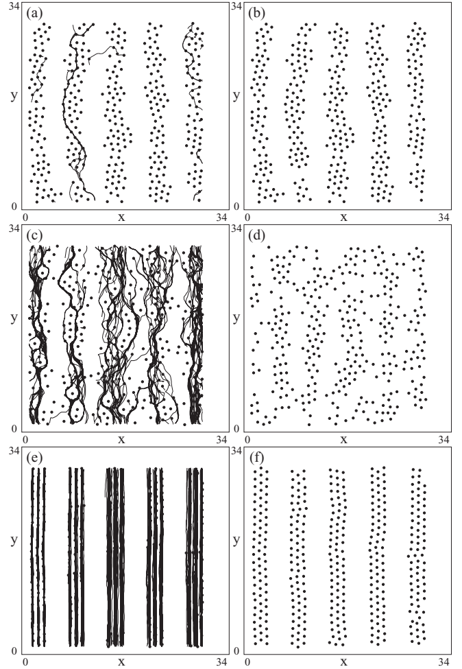
FIG. 3. The particle positions (black dots) and particle trajectories (black lines) for the system in Figs. 2(a) and 2(b) for pulse driving in the y direction. The particle trajectories are traced over equal times in panels (a), (c), and (e). (a) At F_D^y = 0.05 there is a filamentary flow pattern along the stripes. (b) A snapshot of only the particle positions from (a) shows that the stripe structure is partially preserved. (c) At F_D^y = 0.125 , fluctuating plastic flow occurs in which channels of moving particles intertwine and mix while other particles remain pinned. (d) The particle positions only for the system in (c) indicate that the stripe structures are completely disordered. (e) At F_D^y = 0.2 , above the peak in d\langle V_y \rangle/dF_D^y shown in Fig. 2(b), all the particles are moving in an ordered stripe phase. (f) A plot of only the particle positions from (e) shows the ordered stripes.
