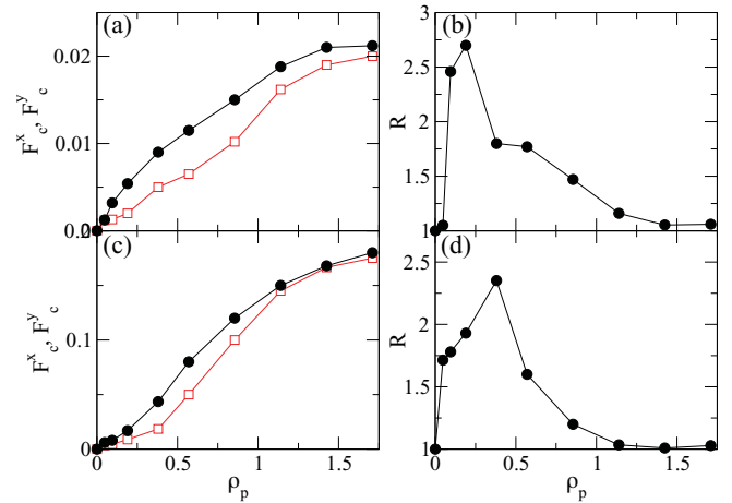
FIG. 15. (Color online) (a) F_c^x (filled circles) and F_c^y (open squares) vs \rho_p for a system with F_p = 0.225 and R_p = 0.3 . (b) The corresponding R = F_c^x/F_c^y vs \rho_p shows that at large \rho_p the anisotropy is reduced. (c) F_c^x (filled circles) and F_c^y (open squares) vs \rho_p for a system with F_p = 0.7 and R_p = 0.3 . (d) The corresponding R vs \rho_p . Here the anisotropy drops nearly to R = 1 at high \rho_p .
