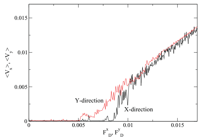
FIG. 12. (Color online) A combined plot of \langle V_x \rangle vs F_D^x (dark line) and \langle V_y \rangle vs F_D^y (lighter line) for a system with \rho_p = 0.38 , a lower F_p = 0.225 , and a swept drive. The depinning in the x direction is accompanied by plastic distortions and the partial breaking apart of the stripe structure. Depinning in the y direction occurs by the sliding of stripes past one another in a manner similar to that illustrated in the inset of Fig. 9.
