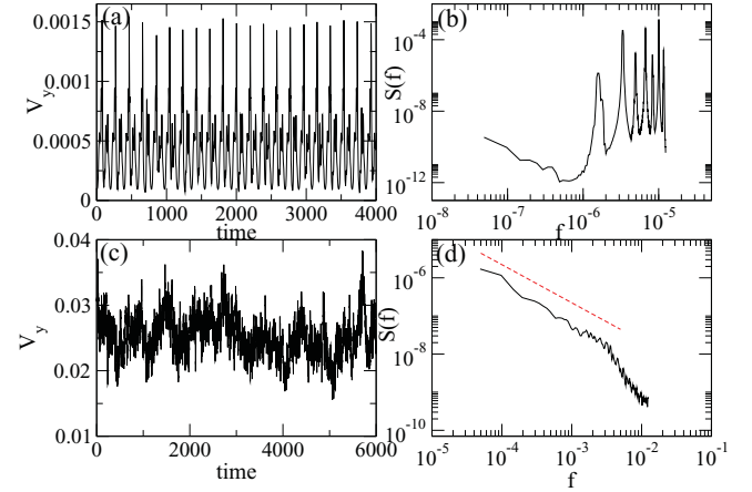
FIG. 17. (Color online) (a) The time series of V_y for a system with F_p = 0.9 , \rho_p = 0.36 , R_p = 0.2 , and F_D^y = 0.04 . For these parameters, the particles move in stationary plastic filaments, producing a periodic time-of-flight signal. (b) The power spectrum S(f) of the time series in (a) showing the characteristic peaks from the periodic signal. Here, f is in units of inverse simulation time steps. (c) Time series of V_y for the same system at F_D^y = 0.12 in the strongly fluctuating plastic flow regime. (d) The corresponding S(f) has a 1/f feature at low frequencies as indicated by the dashed line.
