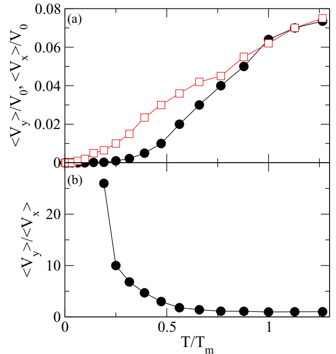
FIG. 19. (Color online) (a) \langle V_x \rangle / V_0 (filled circles) and \langle V_y \rangle / V_0 (open squares) vs T/T_m for a system with \rho_p = 0.36 , R_p = 0.2 , and F_p = 0.7 at applied drives of F_D^x = 0.09 and F_D^y = 0.09 , respectively. Here T_m is the temperature at which the stripes melt in the absence of pinning and V_0 is the velocity at which the particles would move in the absence of pinning. Anisotropic transport occurs for T/T_m < 1.0 . (b) Velocity anisotropy ratio \langle V_y \rangle / \langle V_x \rangle vs T/T_m for the same system shows a diverging anisotropy at low temperatures.
