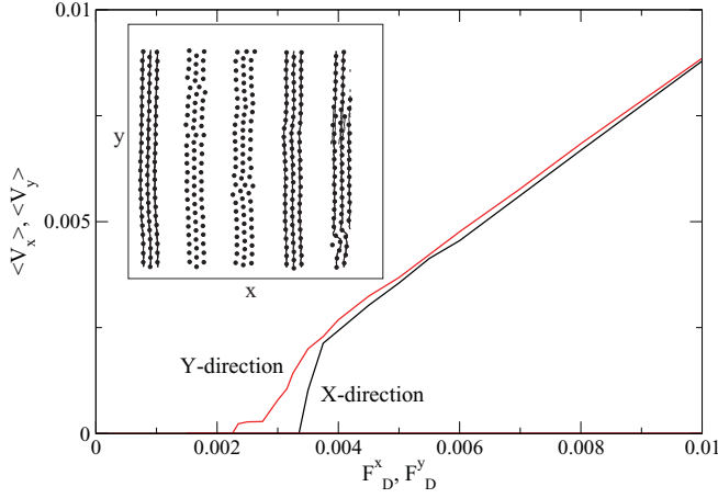
FIG. 9. (Color online) A combined plot of \langle V_x \rangle vs F_D^x (dark line) and \langle V_y \rangle vs F_D^y (light line) for the system in Fig. 8 with F_p = 0.125 highlighting the transport anisotropy. Inset: The particle positions (dots) and trajectories (lines) for the system in Fig. 8(a) in the decoupled stripe regime at F_D^y = 0.0025 where a portion of the stripes are moving while others are pinned.
