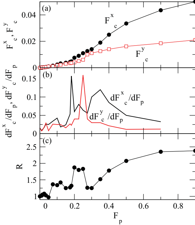
FIG. 13. (Color online) (a) The critical depinning forces F_c^x (filled circles) and F_c^y (open squares) for driving in the x and y directions, respectively, plotted vs F_p . The sharp jumps in the depinning forces are associated with changes from elastic flow to plastic flow and from plastic flow to sliding ordered flow. (b) The corresponding dF_c^x/dF_p vs F_p (dark line) and dF_c^y/dF_p vs F_p (light line) curves more clearly show the onset of the different depinning phases. (c) The anisotropy ratio R = F_c^x/F_c^y vs F_p shows that the change in anisotropy can be associated with different depinning regimes.
