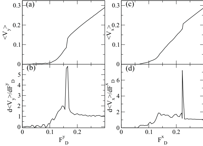
FIG. 2. (a) The average steady state velocity \langle V_y \rangle vs F_D^y for pulse driving in the y direction. We use the same parameters as in Fig. 1 with F_p = 0.9 and \rho_p = 0.38 . Here the drive is suddenly increased from zero to F_D and the system settles into a steady state after a transient time \tau . (b) The corresponding d\langle V_y \rangle/dF_D^y , with a sharp peak indicating the transition to a moving stripe phase for F_D^y \geq 0.165 . (c) \langle V_x \rangle vs F_D^x for the same system. (d) The corresponding d\langle V_x \rangle/dF_D^x vs F_D^x showing a sharp peak at the transition to a perpendicularly translating stripe state.
