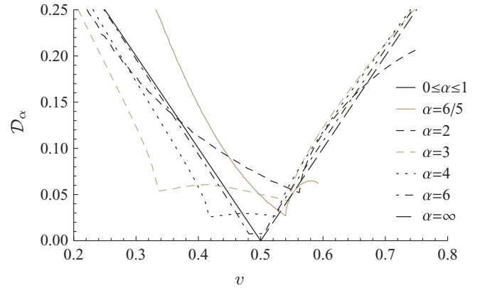
FIG. 6. Asymptotic large- N behavior \mathcal{D}_\alpha of the Hessian determinant, plotted as a function of the potential energy per spin v for various exponents \alpha . Dark lines correspond to values of \alpha for which exact analytic results are available, light lines (for \alpha = 6/5 and \alpha = 3 ) were obtained numerically. The dark solid straight line is obtained analytically for \alpha = 1 , but coincides with the numerical results [and also with the Hadamard bound (39)] for \alpha \in [0, 1] . \mathcal{D}_\alpha vanishes at v = 1/2 for \alpha \in [0, 1] (long-range interactions) as well as for \alpha = \infty (nearest-neighbor interactions). For all finite \alpha > 1 , \mathcal{D}_\alpha is bounded away from zero.
