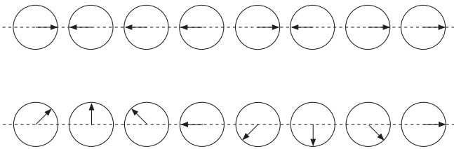
FIG. 1. Sketch of stationary points of the potential V for N = 8 , where \theta_i is the angle between the arrow and the dashed axis. Top: Stationary points where all \theta_i \in \{0, \pi\} . Bottom: Spinwave stationary point (9), where all differences \theta_i - \theta_{i-1} between neighboring angles are equal, with differences chosen such that \theta_0 = \theta_N , in compliance with the periodic boundary conditions.
