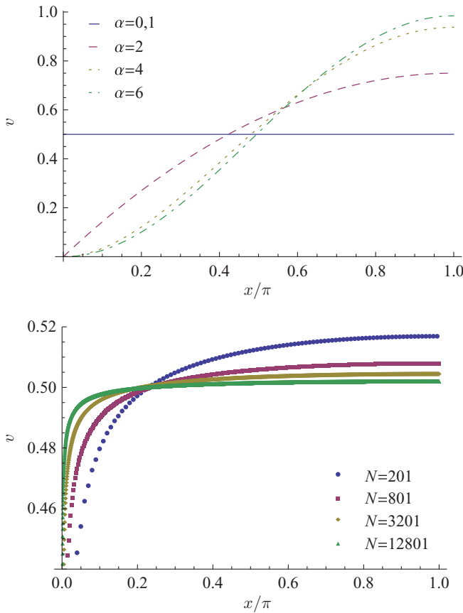
FIG. 2. (Color online) Upper plot: The graph of the potential energy per spin e(x) of a spinwave solution \theta^{(x)} in the thermodynamic limit as given in (12). For a given positive, even \alpha = 2, 4, 6, \dots , the energy values cover densely the entire range of energies per spin accessible to the system in the thermodynamic limit. Lower plot: Potential energy per spin e(x) for \alpha = 1/2 and spinwave stationary points (9), plotted for various system sizes N . With increasing N , the curve approaches a horizontal line of energy 1/2 .
