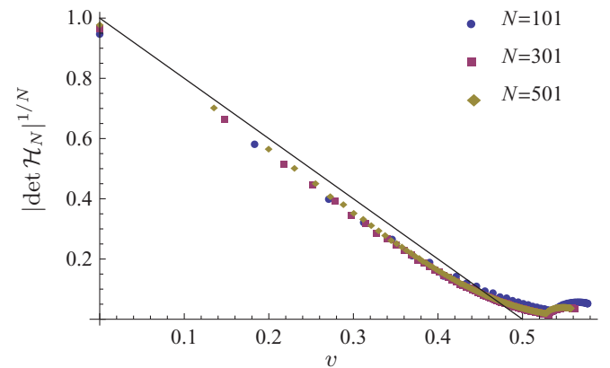
FIG. 3. (Color online) The N th root of the Hessian determinant \det \mathcal{H}_N for \alpha = 1 , evaluated at spinwave stationary points \theta^{(x)} , plotted versus the corresponding potential energy per spin v(x) . With increasing system size N , the numerically computed determinant slowly (logarithmically) approaches the analytic large- N asymptotic result \mathcal{D}_1 (black line).
