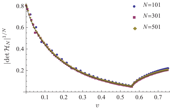
FIG. 5. (Color online) The N th root of the Hessian determinant \det \mathcal{H}_N for \alpha = 2 , evaluated at spinwave stationary points \theta^{(x)} , plotted versus the corresponding potential energy per spin v(x) . Already for moderate system sizes N , the finite-system data are in excellent agreement with the analytic large- N asymptotic result \mathcal{D}_2 (black line).
