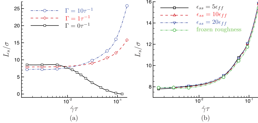
FIG. 4. (Color online) The effect of (a) thermostatting mechanism and (b) wall parameters on the slip length versus shear-rate behavior.
