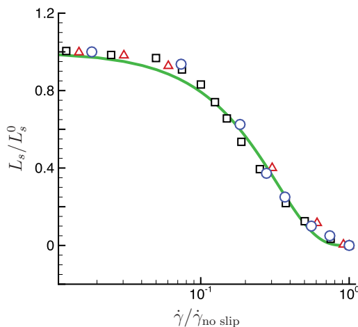
FIG. 6. (Color online) Fit of the slip length: \square \epsilon_{fs} = 0.1 ; \triangle \epsilon_{fs} = 0.2 ; \circ \epsilon_{fs} = 0.3 ; and — the fit (3).
