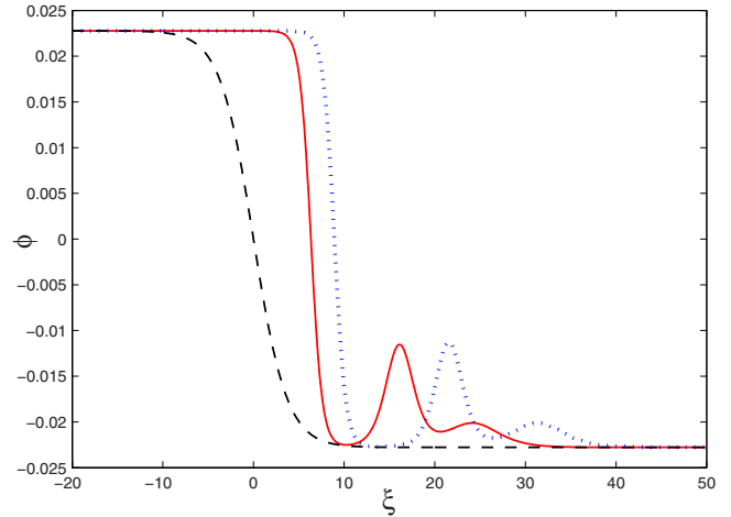
FIG. 1. (Color online) The profiles of the DL shocks for three different times. The initial profile ( \tau=0 ) steepens (dashed line), and simultaneously two solitary waves form in front of the shock (see the solid line for \tau=150 and the dotted line for \tau=200 ).
