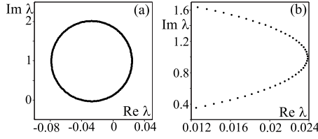
FIG. 2. Spectrum of the origin in the array of delay-coupled N=200 oscillators. The round trip time is T=10 , which corresponds to a small delay \tau=0.05 between the neighboring oscillators. The spectrum is approximated by expression (8). (a) Whole spectrum; (b) zoom of the eigenvalues with the largest real parts. \alpha=-0.99 and \beta=1 .
