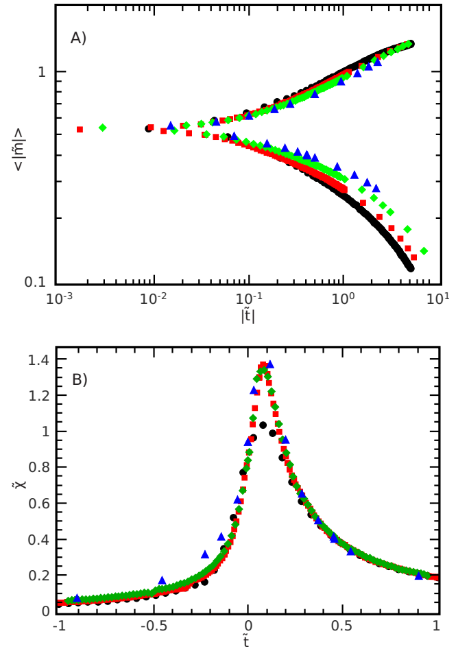
FIG. 3. (Color online) Finite size scaling data collapses for the whole system. The black circles correspond to a size of 59 \times 23 \times 13 , the red squares to a size of 109 \times 43 \times 25 , the green diamonds to a size of 205 \times 83 \times 50 and the blue triangles to a size of 417 \times 167 \times 101 . The critical exponent \nu=2.0 and the critical temperature is T_c=4.50 . (A) Magnetization scaling function \langle |\bar{m}| \rangle vs |\bar{t}| using the long-range order critical exponent \beta=0.18 . (B) Susceptibility scaling function \bar{\chi} vs scaled reduced temperature \bar{t} using the critical exponent \gamma=1.1 .
