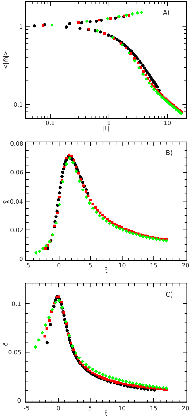
FIG. 2. (Color online) Finite size scaling data collapses for a quasi-two-dimensional layer at the surface of an ordered cylindrical nucleus. The black circles correspond to an x - y cross section circumference of 50, the red squares to a circumference of 102 and the green diamonds to a circumference of 200. The critical exponent \nu=2.0 and the critical temperature is T_c=6.7 . (A) Magnetization scaling function \langle |\bar{m}| \rangle vs |\bar{t}| using the long-range order critical exponent \beta=0.18 . (B) Susceptibility scaling function \bar{\chi} vs scaled reduced temperature \bar{t} using the critical exponent \gamma=1.0 . (C) Specific heat scaling function \bar{c} vs \bar{t} using the critical exponent \alpha=0.10 .
