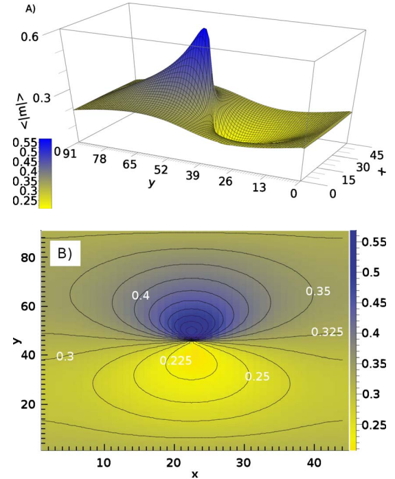
FIG. 1. (Color online) (A) Magnetization order parameter \langle |m| \rangle for the x - y cross section, averaged over sites in the z direction, of a 45 \times 91 \times 40 system at a temperature of 4.49 k_B . The order-enhanced and order-suppressed zones are shown in blue (dark) and yellow (light), respectively. (B) Contour plot of the same data. The contour lines are in a step of 0.025. The innermost line in the blue (dark) order-enhanced region corresponds to 0.55.
