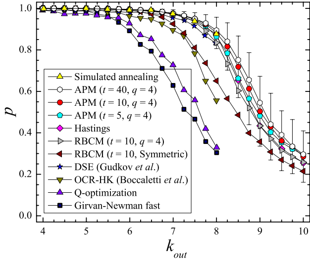
FIG. 1. (Color online) Plot of the percentage of correctly identified nodes p versus the average external degree k_{out} [32]. The average node degree is k=16 . The data for the APM of Eq. (2) and the RBCM of Eq. (7) both use \gamma=\gamma_{RB}=1 . Both models use the algorithm in Sec. III with q=4 by constraint (see text regarding the RBCM/Symmetric data). The APM is at least as accurate as SA (error bars are for t=10 optimization trials), and the RBCM performs excellently also. Each point is an average over 500 runs.
