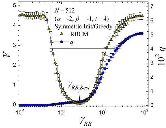
FIG. 10. (Color online) Plot of VI V vs \gamma_{RB} for the RBCM. In Sec. V B, we generate a set of strongly defined communities with varying levels of intercommunity noise k_{out} . Using the greedy algorithm in Sec. III, we compare the accuracy of solutions found with the RBCM to our APM. Since the models operate differently, we compare the results in Figs. 5 and 6 for our APM using \gamma=1 to the best result for the RBCM independently determined for each k_{out} . To this end, we increment \gamma_{RB} by 20 steps per decade and calculate VI for each solution using the known answer . We then select the best \gamma_{RB} corresponding to the lowest VI average. This example is for a system with N=512 nodes (see Fig. 4) with an average external degree k_{out} \approx 10 . See the text regarding other parameters defining the distribution of initial node degrees and community sizes. Each point is an average over 100 graphs.
