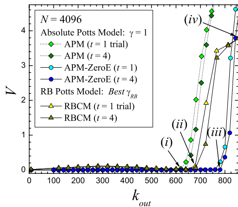
FIG. 12. (Color online) Plot of VI V vs the average external degree k_{out} for the APM and RBCM models. Similar to Sec. V B, we generate strongly defined communities with N=4096 nodes and high levels of intercommunity noise. We use the greedy algorithm in Sec. III for both models. The system is initially assigned a random power-law degree distribution with an exponent \alpha=-2 , maximum degree k_{max}=1200 , and average degree \langle k \rangle_\alpha ( k_{out} \approx \langle k \rangle_\alpha ). Communities are assigned in a power-law distribution with an exponent \beta=-1 , minimum size n_{min}=8 , maximum size n_{max}=24 , and density p_{in}=1 . The APM shows sharp accuracy transitions at (i) near k_{out} \approx 620 (no zero energy moves) and at (iii) near k_{out} \approx 770 (using zero energy moves). These roughly correspond to a similar transition for the RBCM at (ii). See the text regarding (iv). Each point is an average over 25 graphs.
