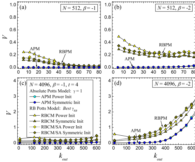
FIG. 6. (Color online) Plot of VI V between solved and known test systems in Sec. VB vs the average external node degree k_{out} . In panels (a) through (d), system sizes are N_{a,b}=512 and N_{c,d}=4096 nodes, respectively. The graphs are solved with the APM and the RBCM using the algorithm in Sec. III with t=4 trials. The constructed configurations are identical to those used in Fig. 5. In this plot, we test two different initial states for the solutions: a symmetric initial state and a random power-law distribution (see text). We use \gamma=1 for the APM on all solutions, and we subjectively choose the best \gamma_{RB} for the RBCM for each k_{out} (see Appendix C). For comparison, the results for SA with t=4 are also depicted and are solved using this best value of \gamma_{RB} . The APM and SA with the RBCM show no difference in accuracy between the symmetric and random initial states. A symmetric state appears to be the favored starting configuration for the RBCM when using a greedy algorithm in this benchmark. In fact, this symmetric initial state allows the RBCM to slightly outperform SA in accuracy (see text). We average over 100 graphs in panels (a) and (b) and 25 graphs in panels (c) and (d).
