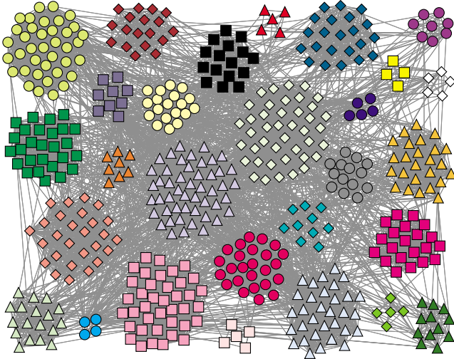
FIG. 4. (Color online) A sample graph with N=512 nodes for the noise test in Sec. VB. In this sample, the node degrees are initially defined in a power-law distribution with an average \langle k \rangle_\alpha = 5.4 , maximum k_{\max} = 100 , and exponent \alpha = -2 . Communities have a power-law distribution of sizes with a minimum n_{\min} = 4 , maximum n_{\max} = 50 , and exponent \beta = -1 . These communities are then strongly defined by connecting all internal community edges ( p_{in} = 1 ).
