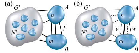
FIG. 8. (Color online) A large graph G has N nodes and three subdivisions depicted, one potentially large subgraph G' with N' nodes and two distinct communities A and B with n and m nodes, respectively. In panel (a), G is unweighted, and communities A and B are joined by l edges. In panel (b), G is a weighted graph. For visualization purposes, solid lines depict weighted edges, dashed lines depict weighted missing links, and the link thickness depicts a relative link weight. Communities A and B are joined by weighted edges with a summed weight of w . Weighted missing links have a summed weight of u . All other graph features are left unspecified but are consistent with the community designations.
