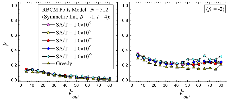
FIG. 11. (Color online) Plot of VI V vs the average external degree k_{out} for the RBCM. In Sec. V B, we generate a set of strongly defined communities with high levels of intercommunity noise. In Figs. 5 and 6, we vary the initial average power-law degree \langle k \rangle_{\alpha} \approx k_{out} and solve the networks using the greedy algorithm in Sec. III and SA where we use a starting temperature of T_0=1.0 \times 10^{-4} for the N=512 node systems. The greedy algorithm initialized into a symmetric initial state ( q_0=N ) outperforms SA in accuracy when using the best \gamma_{RB} (see Appendix C). In these plots, we further examine SA for a range of starting temperatures. Even with significantly higher starting temperatures, SA cannot exceed the accuracy of the greedy algorithm in this problem.
