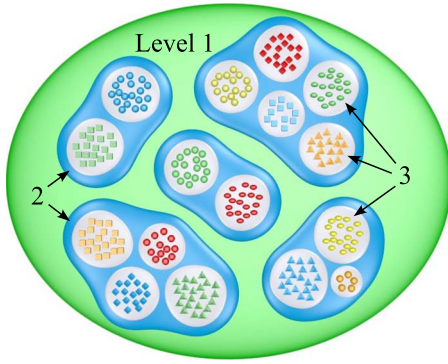
FIG. 2. (Color online) The figure depicts a simulated three-level heterogeneously sized hierarchy with N=256 nodes [22,35]. The innermost level 3 has q_3=16 communities with a randomly assigned average density of \bar{p}_3=0.90 . The intermediate level 2 has q_2=5 communities and an average density of \bar{p}_2=0.47 that is constructed by connecting the constituent level 3 subgroups at an intercommunity edge density of p_2=0.3 . Level 1 is the completely merged system with an average density of \bar{p}_1=0.18 , and it is constructed by connecting nodes in different level 2 communities with an intercommunity edge density of p_1=0.1 .
