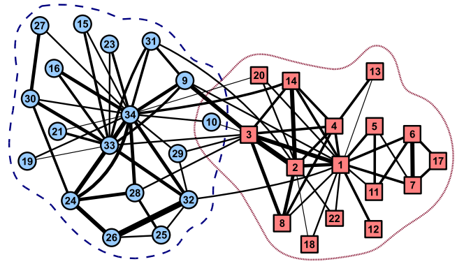
FIG. 9. (Color online) Graph depicts the Zachary karate club [52] solved with the APM using weighted edges (relative line thickness), \gamma=1 , and q=2 communities by constraint. All nodes except 10 are correctly assigned. By our analysis, this node appears frequently in both groups (see text).
