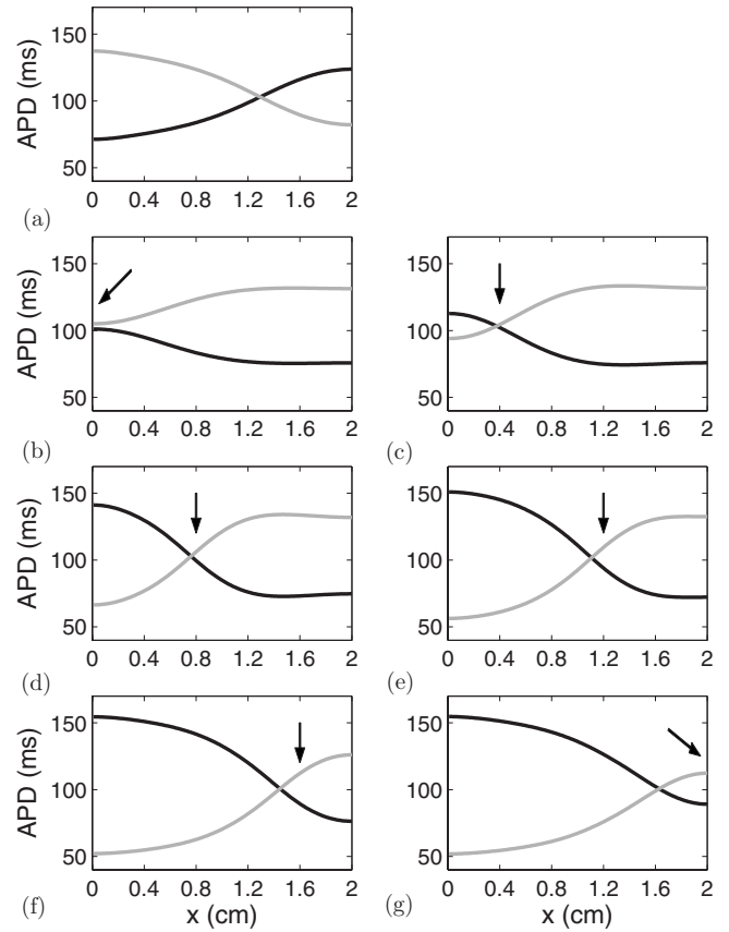
FIG. 3. Off-site control of spatially discordant alternans in coupled maps model with T^* = 140 ms. (a) No control and (b)–(g) control at locations x_r = 0.0, 0.4, 0.8, 1.2, 1.6, and 2.0 cm (indicated by arrows).
