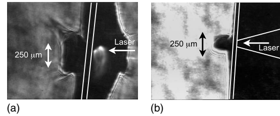
FIG. 2. Shadowgrams of 4 \mu\text{m}/0.2 \mu\text{m}/4 \mu\text{m} CH/Al/CH slab targets without (a) and with (b) a plastic guide cone attached. The shadowgrams were taken 400 \text{ ps} after the main interaction. The original target position is marked on each shadowgram.
