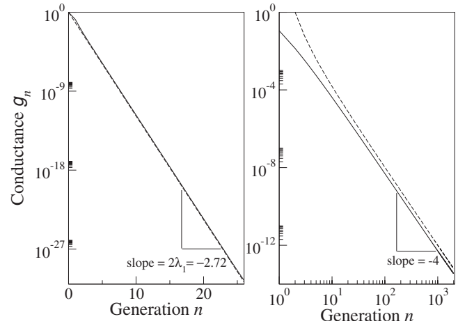
FIG. 3. Conductance as a function of generation for \epsilon=\frac{1}{4} : ka=0.5 (left panel) and ka=\pi/4 (right panel). Continuous lines represent g_n obtained directly from the map through Eq. (5) while dotted lines correspond to g_n = \exp(2\lambda_1 n) and g_n = \exp_{3/2}(2\lambda_{3/2} n) for left panel and right panel, respectively. The two curves in right panel differ because of a proportionality factor [see Eq. (14)].
