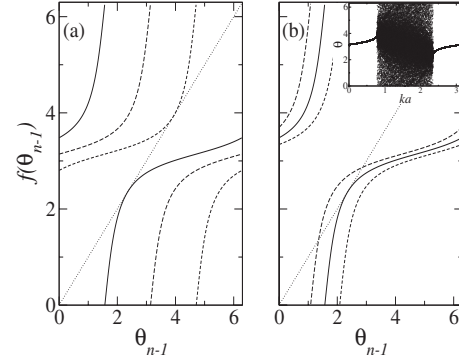
FIG. 2. f(\theta_n) of Eq. (6) for \epsilon = \frac{1}{4} : (a) ka = \pi/4 (dashed line), 2\pi/4 (long dashed line), and 3\pi/4 (continuous line) and (b) ka = 2.6 (long dashed line), 3\pi/4 (continuous line), and 2.1 (dashed line). The dotted lines correspond to the identity. Inset: periodic and chaotic attractors.
