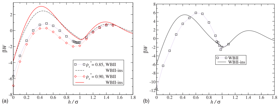
FIG. 11. (Color online) Depletion potential between two solutes, comparison between explicit FMT-WBII data and the insertion route. Left panel: solute-solvent size ratio of 5 and solvent densities \rho_s^*=0.85 and 0.9. Right panel: size ratio 10 and \rho_s^*=0.85 .
