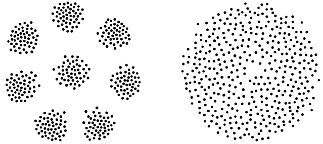
FIG. 1. Layouts with small LinLog energy ( a-r=1 ) and with small Fruchterman-Reingold energy ( a-r=3 ) of a pseudorandom network with eight clusters (intracluster density 1.0, expected intercluster density 0.2).
