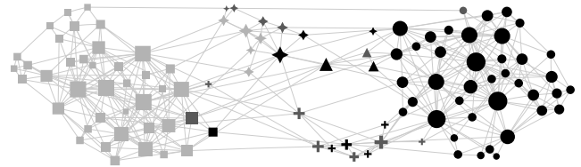
FIG. 5. (0, -2) -energy layout and modularity clustering of the book copurchase network. The modularity is 0.527. Shades represent the classification as liberal (light gray), neutral (dark gray), or conservative (black).
