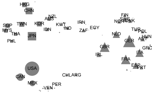
FIG. 7. (0, -1) -energy layout and modularity clustering of the world trade network. The modularity of the clustering is 0.275. (The edges are elided to avoid clutter.)
