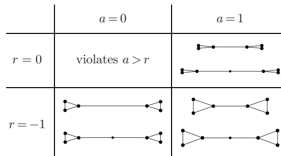
FIG. 2. Layouts with optimal (a, r) energy for different values of a and r . All vertices and edges have weight 1, except for the small vertex between the triangles which has weight 0.
