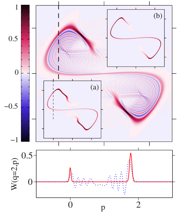
FIG. 4. (Color online) Wigner distribution (top panel) and classical distribution [inset (a)] immediately before the kick n=7 for \eta = \sqrt{2\hbar_{\text{eff}}} = 0.125 and diffusion constant D = 9 \times 10^{-5} . Inset (b): Wigner distribution immediately before the kick n=8 for \eta = \sqrt{2\hbar_{\text{eff}}} = 0.0256 and diffusion constant D = 9 \times 10^{-5} . Bottom panel: Wigner distribution (blue dotted line) and classical distribution (red solid line) evaluated on (q = -2, p) (dashed lines in the top panel).
