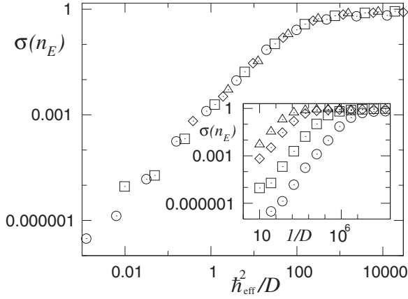
FIG. 3. The measure \sigma(n_E) (see text) of the differences between the quantum and classical Renyi entropies. The initial state is a coherent state centered around the origin of phase space with width \Delta q = \Delta p = \eta , with \eta = \sqrt{2\hbar_{\text{eff}}} = 0.5 (triangles), 0.3125 (diamonds), 0.125 (squares), and 0.0625 (circles). For each \hbar_{\text{eff}} the Renyi entropies were computed at the logarithmic time t_E \approx n_E \tau .
