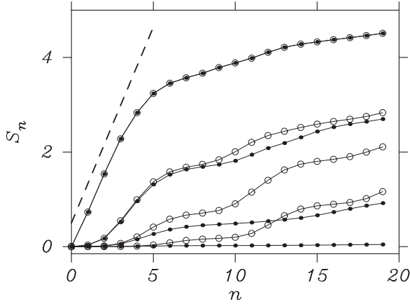
FIG. 1. Quantum (●) and classical (○) Renyi entropy as a function of the number of the kicks for the KHO with K=2 and \eta = \sqrt{\hbar_{\text{eff}}}/2=0.125 . From bottom to top, the diffusion constants are D=2.56 \times 10^{-7} , 6.4 \times 10^{-6} , 9 \times 10^{-5} , and 4 \times 10^{-3} . The dashed line is a linear function with a slope given by the logarithm of the classical expansion coefficient at (q,p)=(0,0) .
