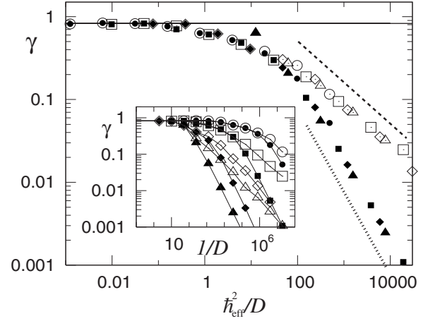
FIG. 2. Slope \gamma of the linear growth of the quantum (solid symbols) and classical (open symbols) Renyi entropies as a function of \hbar_{\text{eff}}^2/D (main plot) and 1/D (inset) ( D is the diffusion constant) for \eta = \sqrt{\hbar_{\text{eff}}}/2=0.5 (triangles), 0.3125 (diamonds), 0.125 (squares), and 0.0625 (circles). We have also plotted the functions \gamma \propto D/\hbar_{\text{eff}}^2 (dotted line) and \gamma \propto \sqrt{D}/\hbar_{\text{eff}} (dashed line). See text for details.
