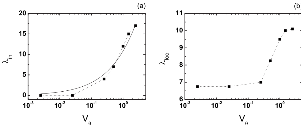
FIG. 9. (a) Width of the inertial zone \lambda_{in} as a function of V_\theta , as deduced from Eq. (6) and Fig. 3(a). The solid line represents the function \lambda_{in} = 50(\sqrt{1 + 0.5V_\theta^{0.57}} - 1) . (b) Width of the localization zone \lambda_{loc} as a function of V_\theta . Geometry R_{50} .
