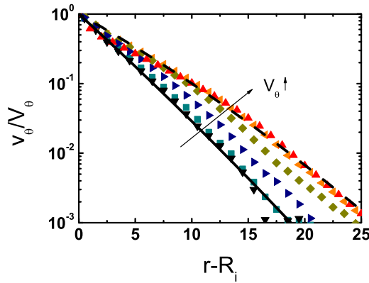
FIG. 4. (Color online) Influence of the shear velocity V_\theta on the velocity profiles v_\theta(r) (semilogarithmic scale). ( \nabla ) V_\theta=0.0025 , ( \blacksquare ) V_\theta=0.25 , ( \blacktriangleright ) V_\theta=0.5 , ( \blacklozenge ) V_\theta=1.0 , ( \blacktriangleleft ) V_\theta=1.5 , ( \blacktriangle ) V_\theta=2.5 . The solid line indicates the function v_\theta/V_\theta = \exp[-0.34(r-R_i) - 0.0015(r-R_i)^2] and the dashed one the function v_\theta/V_\theta = \exp[-0.21(r-R_i) - 0.002(r-R_i)^2] . Geometry R_{50} .
