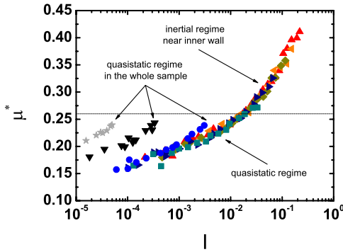
FIG. 10. (Color online) Effective friction \mu^* as a function of the inertial number I ( \star ) V_\theta=0.00025 , ( \blacktriangledown ) V_\theta=0.0025 , ( \bullet ) V_\theta=0.025 , ( \blacksquare ) V_\theta=0.25 , ( \blacktriangleright ) V_\theta=0.5 , ( \blacklozenge ) V_\theta=1.0 , ( \blacktriangleleft ) V_\theta=1.5 , ( \blacktriangle ) V_\theta=2.5 . The solid line corresponds to \mu^*=0.26 . Geometry R_{50} .
