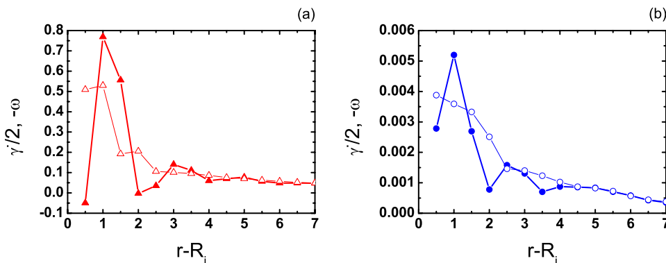
FIG. 5. (Color online) Influence of the inner wall on the collapse between the average angular velocity \omega(r) (hollow symbols) and the shear rate \dot{\gamma}(r) (full symbols) (a) V_\theta=2.5 and (b) V_\theta=0.025 . Geometry R_{50} .
