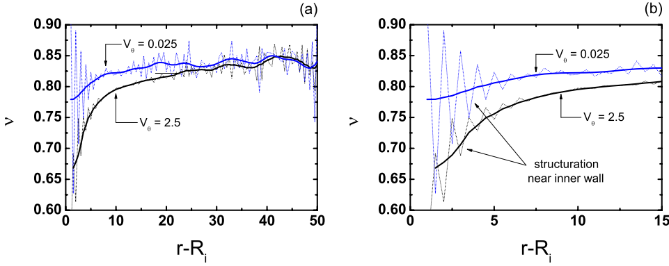
FIG. 6. (Color online) Influence of shear velocity V_\theta on the structuration near the inner wall. Solid fraction profiles \nu(r) (a) in the whole system and (b) in the region close to the inner wall. The solid line is an average over 3d , while the dotted line is an average over 0.5d . Geometry R_{50} .
