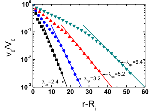
FIG. 18. (Color online) Characteristic length \lambda_{\text{qs}} obtained from the velocity profiles in the quasistatic zone. Different geometries: (■) R_{25} , (●) R_{50} , (▲) R_{100} , (▼) R_{200} . V_\theta = 2.5 .
