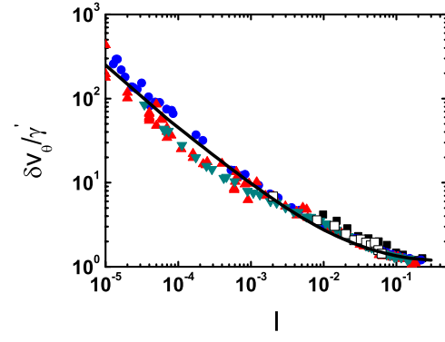
FIG. 15. (Color online) Relative fluctuations as a function of the inertial number I [the solid line represents the function \delta v_\theta / \dot{\gamma} = 1 + 0.07I^{-0.7} ]. (■) R_{25} , (●) R_{50} , (▲) R_{100} , (▼) R_{200} , □ plane shear [4]. V_\theta = 2.5 .
