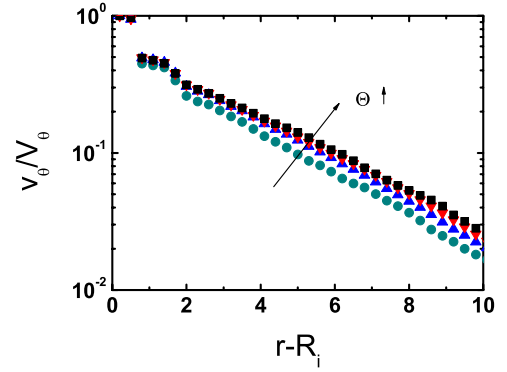
FIG. 21. (Color online) Velocity profiles v_\theta(r)/V_\theta for different values of \Theta rad. (●) \Theta = \pi/16 , (▲) \Theta = \pi/8 , (▼) \Theta = \pi/2 , (■) \Theta = 2\pi . R_i = 25 , R_o = 50 , V_\theta = 2.5 .
