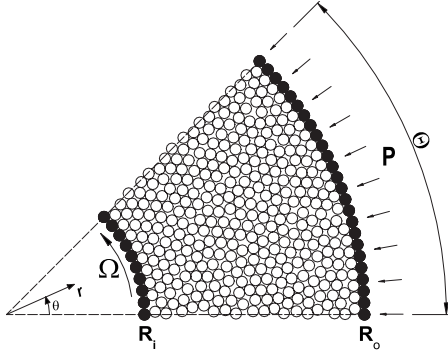
FIG. 1. Annular shear geometry (black grains constitute the rough walls).
