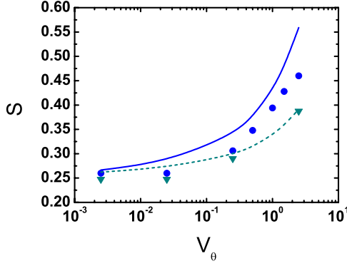
FIG. 17. (Color online) Shear stress at the wall S as a function of the wall velocity V_\theta . Comparison between the measurements: (●) R_{50} and (▼) R_{200} and the predictions of Eq. (13). The solid and dashed line, respectively, indicate the results for R_{50} and R_{200} .
