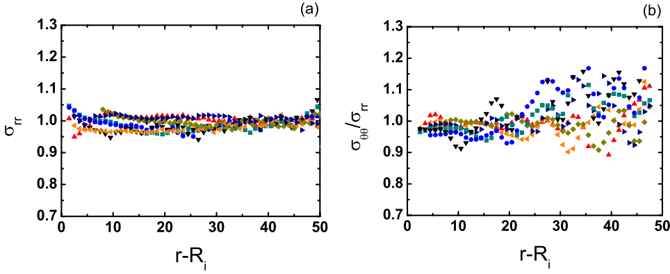
FIG. 2. (Color online) (a) Normal stress \sigma_{rr}(r) and (b) ratio between the normal and the orthonormal stresses \sigma_{\theta\theta}/\sigma_{rr}(r) profiles for different shear velocities. ( \nabla ) V_\theta=0.0025 , ( \bullet ) V_\theta=0.025 , ( \blacksquare ) V_\theta=0.25 , ( \blacktriangleright ) V_\theta=0.5 , ( \blacklozenge ) V_\theta=1.0 , ( \blacktriangleleft ) V_\theta=1.5 , ( \blacktriangle ) V_\theta=2.5 . Geometry R_{50} .
