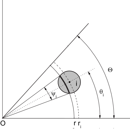
FIG. 23. Various quantities associated to a grain i .
