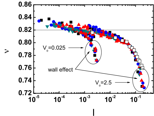
FIG. 12. (Color online) Dynamic dilatancy law in semilogarithmic scale. Different geometries: ( \blacksquare ) R_{25} , ( \bullet ) R_{50} , ( \blacktriangle ) R_{100} , ( \blacktriangledown ) R_{200} . Comparison with plane shear [4] ( \square ). The dashed line corresponds to \nu_{\max}=0.82 .
