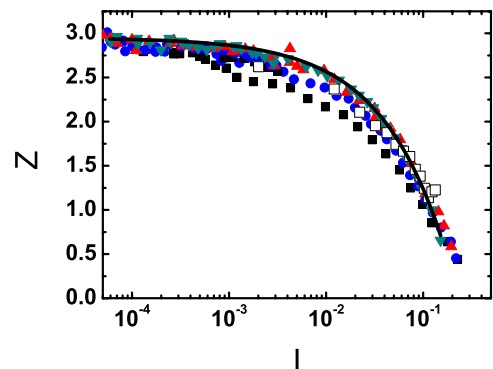
FIG. 13. (Color online) Coordination number Z as a function of the inertial number I (the solid line represents the function Z = 2.95 - 7.65I^{0.65} ) for different geometries. ( \blacksquare ) R_{25} , ( \bullet ) R_{50} , ( \blacktriangle ) R_{100} , ( \blacktriangledown ) R_{200} , ( \square ) plane shear [4]. V_\theta=2.5 .
