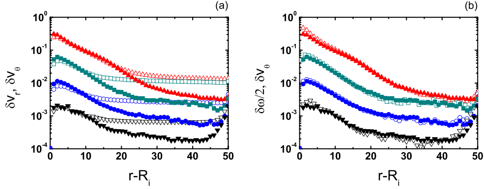
FIG. 26. (Color online) (a) Comparison between the profiles of the fluctuations of the radial velocity \delta v_r (hollow symbols) and of the orthonormal velocity \delta v_\theta (full symbols). (b) Comparison between the profiles of the fluctuations of the angular velocity \delta\omega/2 (hollow symbols) and of the orthonormal velocity \delta v_\theta (full symbols) for different wall velocities V_\theta : ( \nabla , \blacktriangledown ) V_\theta=0.0025 , ( \circ , \bullet ) V_\theta=0.025 , ( \square , \blacksquare ) V_\theta=0.25 , ( \triangle , \blacktriangle ) V_\theta=2.5 . Geometry R_{50} .
