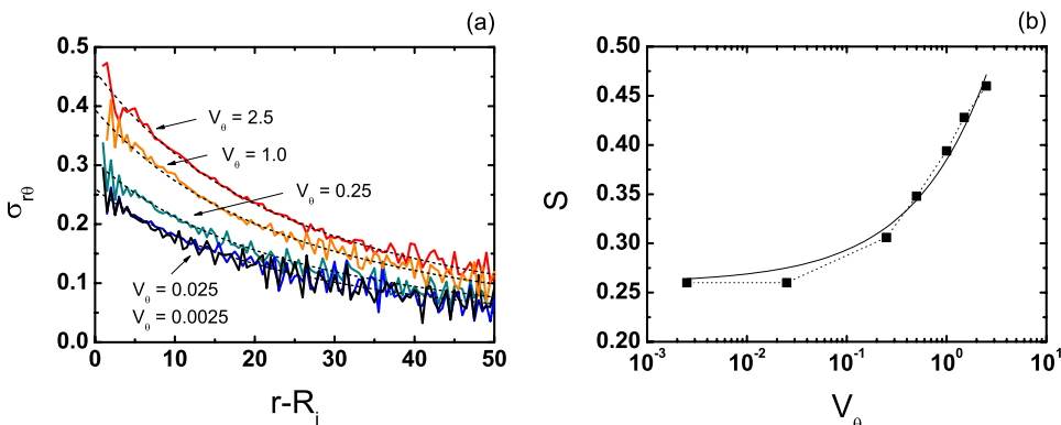
FIG. 3. (Color online) (a) Shear stress profiles \sigma_{r\theta}(r) (solid lines) and fit according to Eq. (3) (dashed lines) for different wall velocities V_\theta . (b) Shear stress at the inner wall S as a function of V_\theta (semilogarithmic scale). The solid line represents the function S = 0.26 + 0.13V_\theta^{0.57} . Geometry R_{50} .
