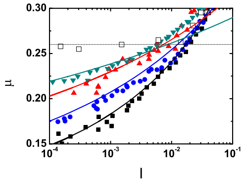
FIG. 19. (Color online) Effective friction \mu^* as a function of the inertial number I , in the quasistatic zone. Comparison between the measurements: (■) R_{25} , (●) R_{50} , (▲) R_{100} , (▼) R_{200} , (□) plane shear [4] and the prediction of Eq. (18) (solid lines). The dashed line indicates \mu_{\min}^* = 0.26 . V_\theta = 2.5 .
