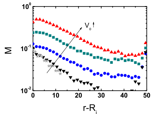
FIG. 25. (Color online) Influence of shear velocity V_\theta on the mobilization of friction profiles M(r) . ( \star ) V_\theta=0.00025 , ( \nabla ) V_\theta=0.0025 , ( \bullet ) V_\theta=0.025 , ( \blacksquare ) V_\theta=0.25 , ( \circ ) V_\theta=2.5 . Geometry R_{50} .
