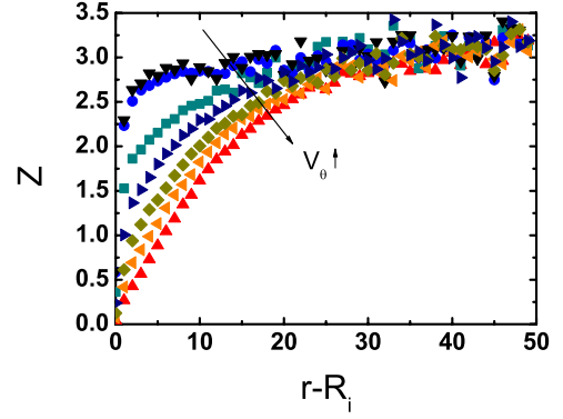
FIG. 24. (Color online) Influence of shear velocity V_\theta on the coordination number profiles Z(r) . ( \nabla ) V_\theta=0.0025 , ( \bullet ) V_\theta=0.025 , ( \blacksquare ) V_\theta=0.25 , ( \blacktriangleright ) V_\theta=0.5 , ( \blacklozenge ) V_\theta=1.0 , ( \blacktriangleleft ) V_\theta=1.5 , ( \blacktriangle ) V_\theta=2.5 . Geometry R_{50} .
