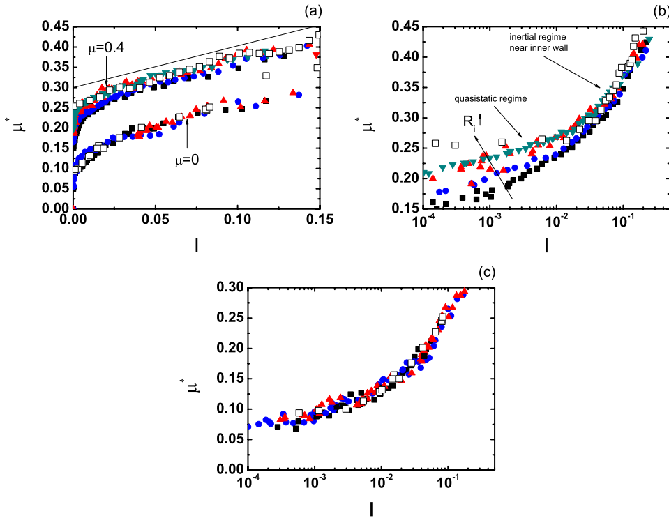
FIG. 8. (Color online) Dynamic friction law (a) in linear scale (the solid line indicates a slope \approx 1 ) for particle coefficient of friction \mu=0 and \mu=0.4 . Dynamic friction law in semilogarithmic scale for (b) \mu=0.4 and (c) \mu=0 . Different geometries: R_{25} , R_{50} , R_{100} , R_{200} . V_\theta=2.5 . Comparison with plane shear [4] ( \square ).
