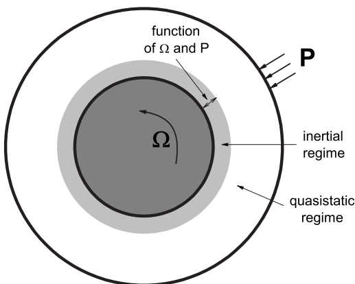
FIG. 7. Inertial and quasistatic zones.
