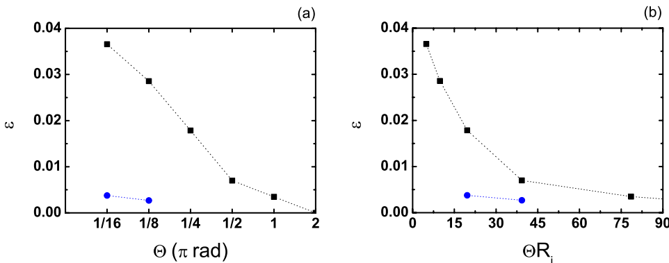
FIG. 22. (Color online) Relative error \varepsilon on the orthoradial velocity v_\theta ( V_\theta = 2.5 ), (a) as function of \Theta , (b) as function of the inner wall length \Theta R_i . (■) R_i = 25 and R_o = 50 , (●) R_i = 100 , and R_o = 200 .
