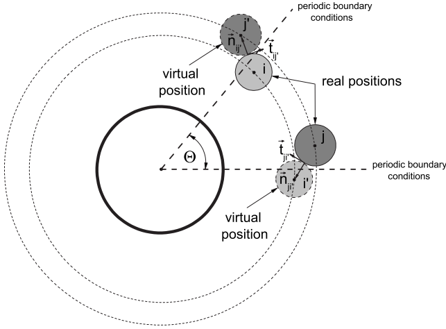
FIG. 20. Periodic boundary conditions.
