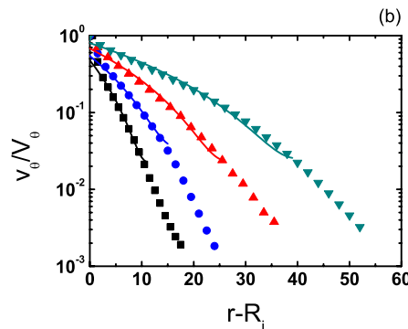
FIG. 16. (Color online) (a) Influence of the geometry on (■) V_\theta^+ / V_\theta (fit) and (□) S (measurement) ( V_\theta = 2.5 ). (b) Velocity profiles: comparison between the measurements (■) R_{25} , (●) R_{50} , (▲) R_{100} , (▼) R_{200} , and the prediction of Eq. (11) (solid lines). The velocity profiles are limited to the steady zone R_i \rightarrow R_i + R_{\text{steady}} ( V_\theta = 2.5 ).
