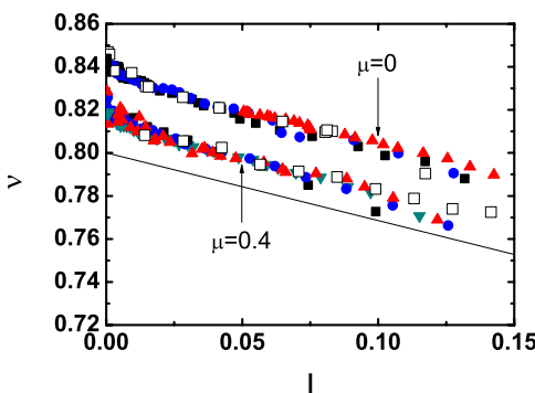
FIG. 11. (Color online) Dynamic dilatancy law (the solid line indicate a slope \approx -0.37 ) for different geometries: ( \blacksquare ) R_{25} , ( \bullet ) R_{50} , ( \blacktriangle ) R_{100} , ( \blacktriangledown ) R_{200} . Comparison with plane shear [4] ( \square ).
