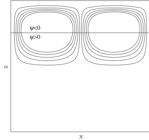
FIG. 4. Streamlines of the critical perturbation at L=0.001 , \bar{\psi}=0.25 , and A=1 , the point denoted in Fig. 3.
