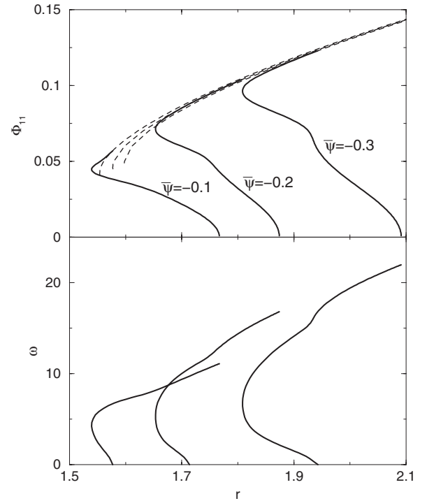
FIG. 11. Bifurcation diagrams for stationary rolls (dashed, upper branch only) and TWs (solid) for the parameters \sigma=10 , L=0.01 , k=5 , A=1 , and three different \bar{\psi} . Plotted are the leading \Phi amplitude (above) and frequency (below) as a function of the reduced heating rate.
