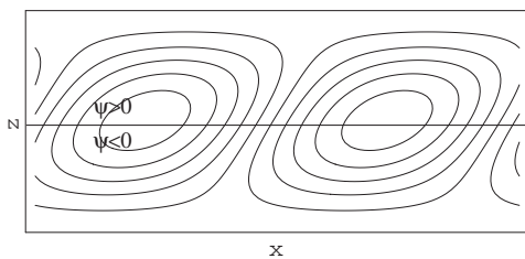
FIG. 6. Streamlines at L=0.001 , \bar{\psi}=-0.025 , \sigma=10 , and A=1 , the point denoted in Fig. 5, in the laboratory frame.
