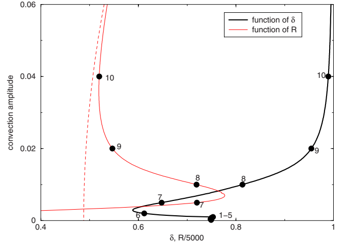
FIG. 8. (Color online) Convection amplitude versus R and versus the height of the virtual cell in comparison. Parameters are \bar{\psi}=0 , A=1 , L=0.01 , \sigma=10 , and k=5 . The numbered dots refer to Fig. 9.
