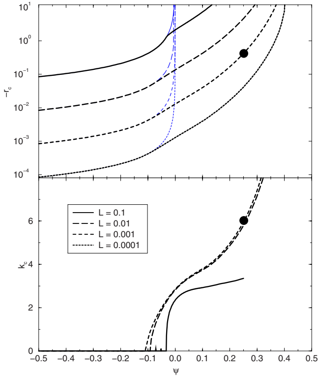
FIG. 3. (Color online) The values (r_c, k_c) for heating from above as a function of \bar{\psi} for four different L and A=1 (thick black lines) compared to A=0 (thin blue lines). The two dots denote the location of the structure in Fig. 4 in parameter space. k_c for L=0.0001 is again not plotted for the same reasons as in Fig. 1. For A=0 it is k_c \equiv 0 and therefore only the curves for A=1 are shown in the lower plot.
