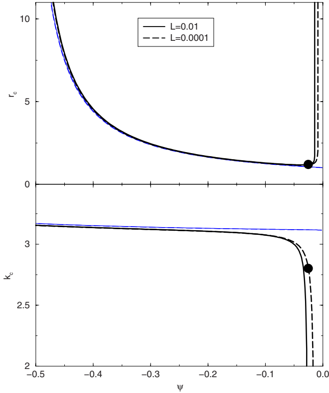
FIG. 5. (Color online) The values (r_c, k_c) for heating from below and oscillatory convection as a function of \bar{\psi} for \sigma=10 , two different L , and A=1 (thick black lines) compared to A=0 (thin blue lines). The two dots denote the location of the structure in Fig. 6 in parameter space.
