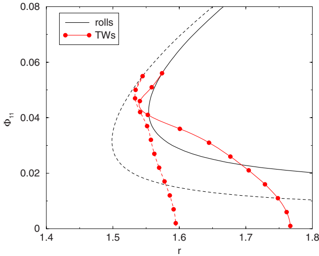
FIG. 10. (Color online) Bifurcation diagrams for stationary rolls and TWs for the parameters \sigma=10 , L=0.01 , \bar{\psi}=-0.1 , k=5 , and A=0 (dashed) and A=1 (solid). Dots on the TW branches denote structures with \omega=0 (highest point) to \omega=11 (lowest point) in steps of \Delta\omega=1 .
