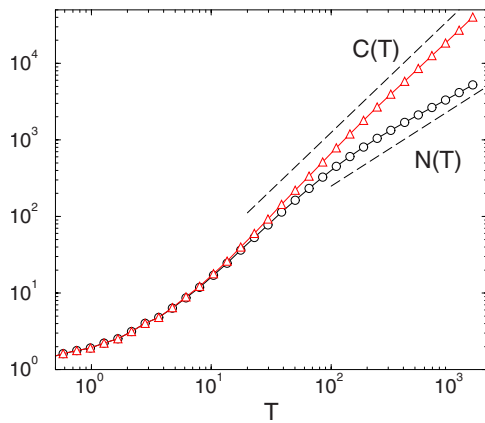
FIG. 2. (Color online) Number of moving spheres N(T) and number of collisions C(T) versus scaled time T=n^{1/2}v_0t in two dimensions for volume fraction 0.2. The dashed lines have slopes 1 and 3/2 as predicted by theory.
