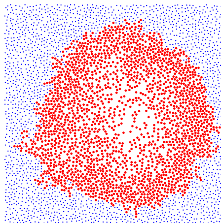
FIG. 1. (Color online) Collision cascade in two dimensions at volume fraction \rho=0.4 and dimensionless time T=n^{1/2}v_0t \approx 197 , with n the number density. Moving spheres are shown actual size (red, inner region) and stationary ones at half radius (blue, outer region). The cascade slowly moves rightward due to a particle initially at the center moving to the right.
