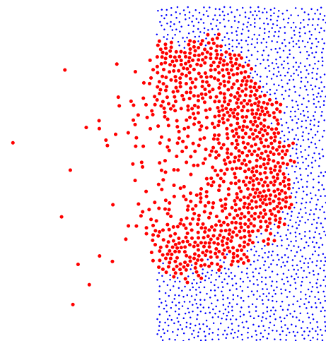
FIG. 4. (Color online) Collision cascade in a two-dimensional half space at volume fraction \rho=0.4 and scaled time T \approx 143 when a particle impacts from the left at t=0 .
