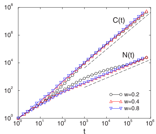
FIG. 3. (Color online) Dependence of N(T) and C(T) versus scaled time T=nv_0t in one dimension on a double logarithmic scale for different widths of the distribution of particle masses. The asymptotic behavior is approached more slowly for narrower mass distributions. The dashed lines have slopes 4/3 and 2/3 as predicted by theory.
