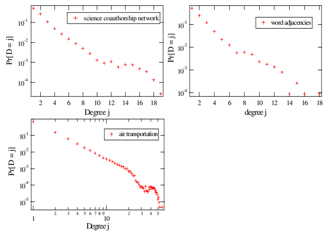
FIG. 10. (Color online) Degree distribution of G_{USPT(\alpha \rightarrow 0)} on top of real network topologies.
