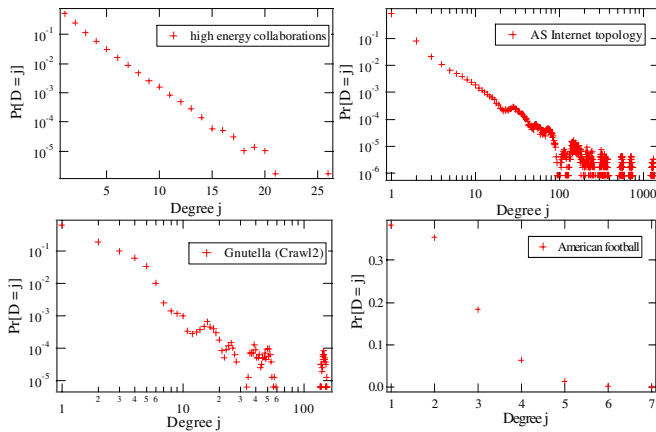
FIG. 8. (Color online) Degree distribution of G_{USPT(\alpha \rightarrow 0)} on top of real network topologies.
