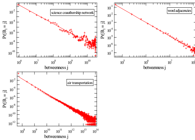
FIG. 7. (Color online) Betweenness distribution (+) of G_{USPT(\alpha \rightarrow 0)} on top of real network topologies. The line is the linear curve fitting.
