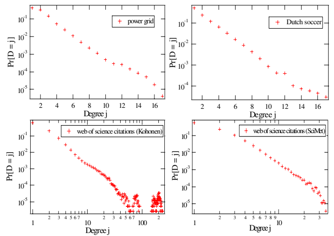
FIG. 9. (Color online) Degree distribution of G_{USPT(\alpha < \alpha_c)} on top of real network topologies.
