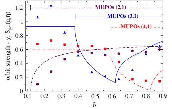
FIG. 5. (Color online) Semiclassical strengths S_{\text{sc}} (lines) compared to the experimental strengths y (symbols). S_{\text{sc}} is given by Eq. (7) and expected from periodic orbit theory, while y is extracted from the length spectra, as shown in Fig. 4. Three orbits are considered: diameter (dotted line and circles), triangle (solid line and triangles), and square (dot-dashed line and squares). The horizontal lines (top) indicate the values of \delta for which the corresponding MUPOs exist.
