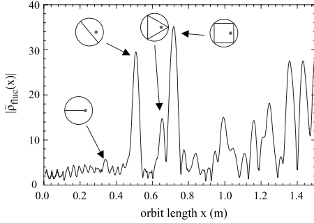
FIG. 4. Experimental length spectrum of the annular billiard for \delta=0.48 . Peaks associated with four periodic orbits are indicated: the shortest one is unstable, the diameter and triangle are MUPOs, and the square is inside the regular region.
