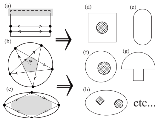
FIG. 1. Adding local perturbations to integrable billiards, as those shown in (a)–(c), one obtains frequently studied chaotic billiards, such as those shown in (d)–(h). The gray regions of the (a) rectangular, (b) circular, and (c) elliptical billiards are defined in such a way that chaotic motion is possible [ a < R in (b) is the radius of the smallest circle that circumscribes all scatterers]. MUPOs are shown here to exist in billiards such as (d) Sinai [1], (e) stadium [2], (f) annular [10], (g) mushroom [11], and (h) elliptical with scatterers [12].
