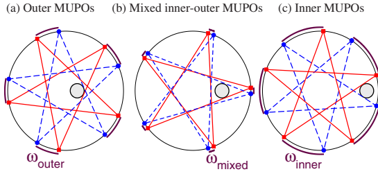
FIG. 3. (Color online) Size w of the families of MUPOs (5, 2) in the annular billiard with r=0.12 : (a) outer MUPOs for \delta=0.2 , (b) mixed inner-outer MUPO for \delta=0.5 , and (c) inner MUPOs for \delta=0.8 . All three kinds of MUPOs may coexist for a fixed \delta . The size w of the families of MUPOs in Eq. (3) is given by the length of the external arcs. MUPOs (5, 2) outside of these regions do not exist since they collide with the inner scatterer.
