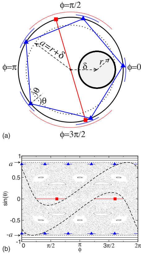
FIG. 2. (Color online) Annular billiard for parameters r=0.35 and \delta=0.5 : (a) configuration space and (b) phase space. MUPOs correspond to the periodic orbits that cross the circle of radius a [dotted line in (a)] but that do not hit the scatterer [region between the dashed lines in (b) in which relation (1) is satisfied]. The symbols \blacksquare and \blacktriangle indicate, respectively, individual orbits belonging to MUPOs (2, 1) and (5, 1) .
