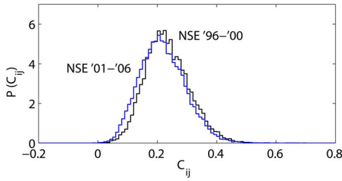
FIG. 8. (Color online) The probability density functions of the elements in the correlation matrix \mathbf{C} for NSE during (a) the period Jan 1996–Dec 2000 and (b) Jan 2001–May 2006. The mean value of the elements of \mathbf{C} for the two periods are 0.23 and 0.21, respectively.
