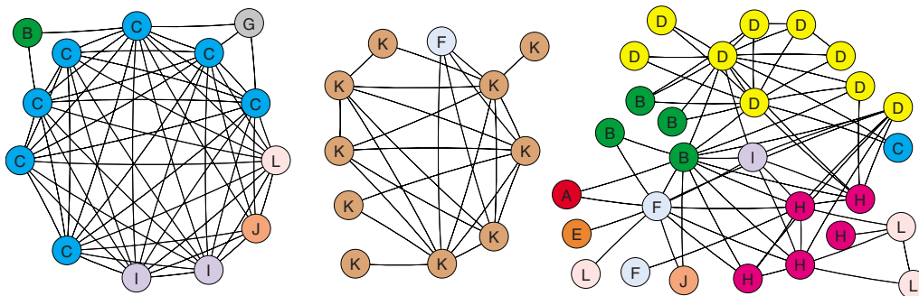
FIG. 7. (Color online) The structure of interaction network in the Indian financial market at threshold c^*=0.09 . The left cluster comprises of mostly technology stocks, while the middle cluster is composed almost entirely of healthcare and pharmaceutical stocks. By contrast, the cluster on the right is not dominated by any particular sector. The node labels indicate the business sector to which a stock belongs and are as specified in the caption to Fig. 3.
