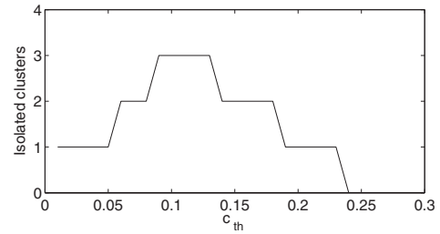
FIG. 6. The number of isolated clusters in the interaction network for NSE stocks as a function of the threshold value c_{\text{th}} . For low c_{\text{th}} the network consists of a single cluster which contains all the nodes, whereas for high c_{\text{th}} the network consists only of isolated nodes.
