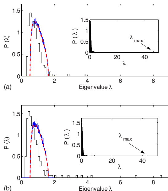
FIG. 2. (Color online) The probability density function of the eigenvalues of the correlation matrix C for NSE (top) and NYSE (bottom). For comparison, the theoretical distribution predicted by Eq. (4) is shown using broken curves, which overlaps with the distribution obtained from the surrogate correlation matrix generated by randomly shuffling each time series. In both figures, the inset shows the largest eigenvalue.
