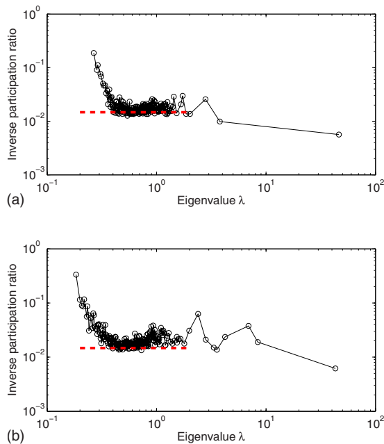
FIG. 4. (Color online) Inverse participation ratio as a function of eigenvalue for the correlation matrix \mathbf{C} of NSE (top) and NYSE (bottom). The broken line indicates the average value of \langle I \rangle = 1.49 \times 10^{-2} for the eigenvectors of a matrix constructed by randomly shuffling each of the N time series.
