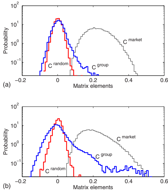
FIG. 5. (Color online) The distribution of elements of correlation matrix corresponding to the market, C^{\text{market}} , the group, C^{\text{group}} , and the random interaction, C^{\text{random}} . For NSE (top) N_g=5 whereas for NYSE (bottom) N_g=10 . The short tail for the distribution of the C^{\text{group}} elements in NSE indicates that the correlation generated by mutual interaction among stocks is relatively weak.
