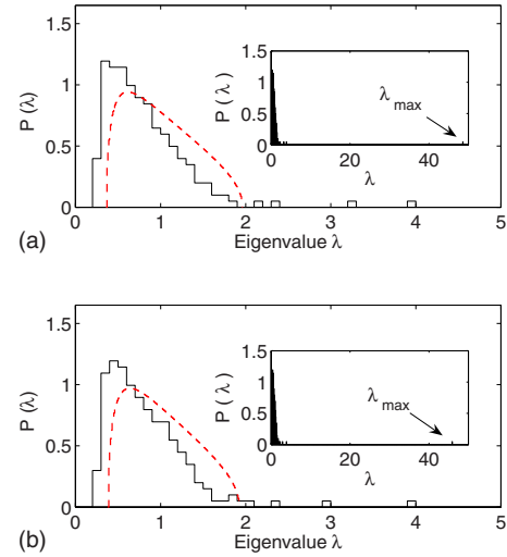
FIG. 9. (Color online) The probability density function of the eigenvalues of the NSE correlation matrix \mathbf{C} for the periods (top) Jan 1996–Dec 2000 and (bottom) Jan 2001–May 2006. For comparison, the theoretical distribution predicted by Eq. (4) is shown using broken curves. In both figures, the inset shows the largest eigenvalue.
