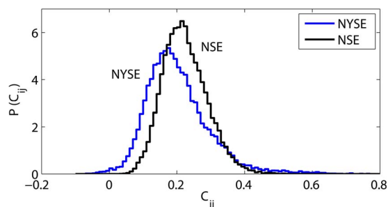
FIG. 1. (Color online) The probability density function of the elements of the correlation matrix C for 201 stocks in the NSE of India and NYSE for the period Jan 1996–May 2006. The mean value of elements of C for NSE and NYSE, \langle C_{ij} \rangle , are 0.22 and 0.20, respectively.
