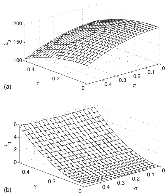
FIG. 10. The variation of the largest (top) and second largest (bottom) eigenvalues of the correlation matrix of simulated return in the two-factor model [Eq. (7)] with the model parameters \gamma and \sigma (corresponding to strength of the sector and idiosyncratic effects, respectively). The matrix is constructed for N=200 stocks each with return time series of length T=2000 days. We assume there to be 10 sectors, each having 20 stocks.
