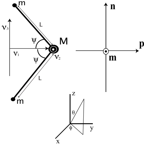
FIG. 1. A schematic representation of the bent-core mesogen [35], with orthonormal molecular axes \{\hat{v}_1, \hat{v}_2, \hat{v}_3\} . The molecular dipole points along \hat{v}_1 , while the molecular body axis lies along \hat{v}_3 ; \hat{v}_2 points into the page. Macroscopically, we define the orthonormal triad \{\mathbf{n}, \mathbf{p}, \mathbf{m}\} with the polar and nematic director fields along \mathbf{p} and \mathbf{n} , respectively.
