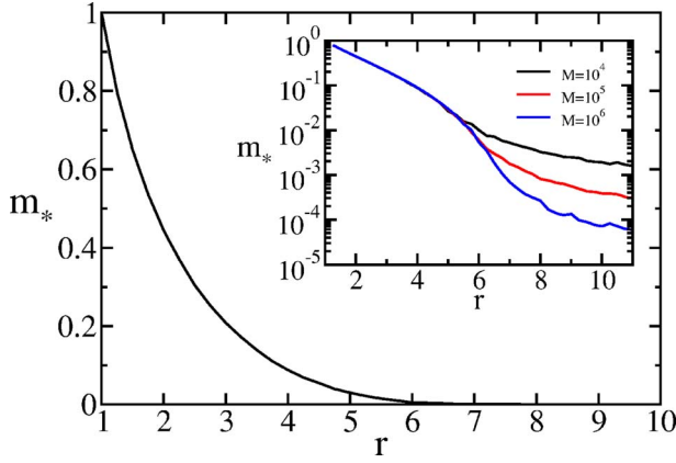
FIG. 4. (Color online) The condensate mass m_* as a function of r obtained from Monte Carlo simulations of the aggregation process (product rate). The results are from a single run with M=10^6 particles. The inset displays the same behavior using a semilog scale. These simulation results represent an average over 100 independent realizations with a varying number of particles.
