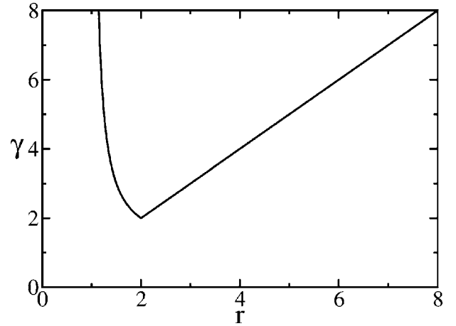
FIG. 2. The exponent \gamma versus r for the sum rate.
