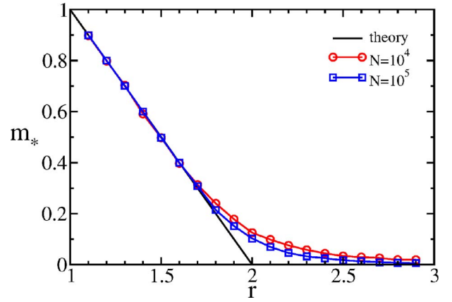
FIG. 1. (Color online) The condensate mass m_* as a function of r for the sum rate. Shown in a solid line is the theoretical prediction (20). Shown in solid lines with symbols are Monte Carlo simulations results for the size of the largest cluster in the system.
