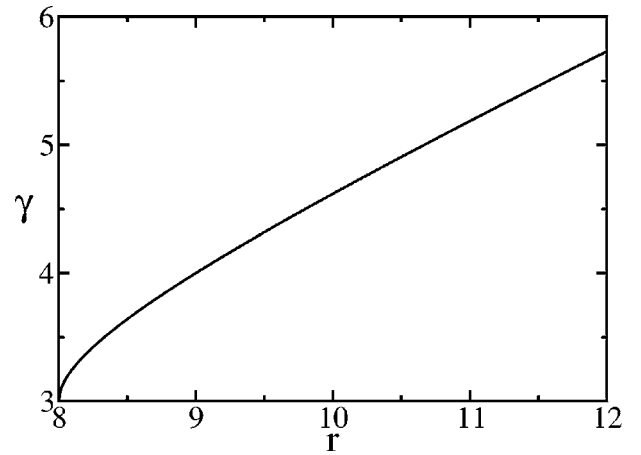
FIG. 3. The exponent \gamma versus r for the product rate.
