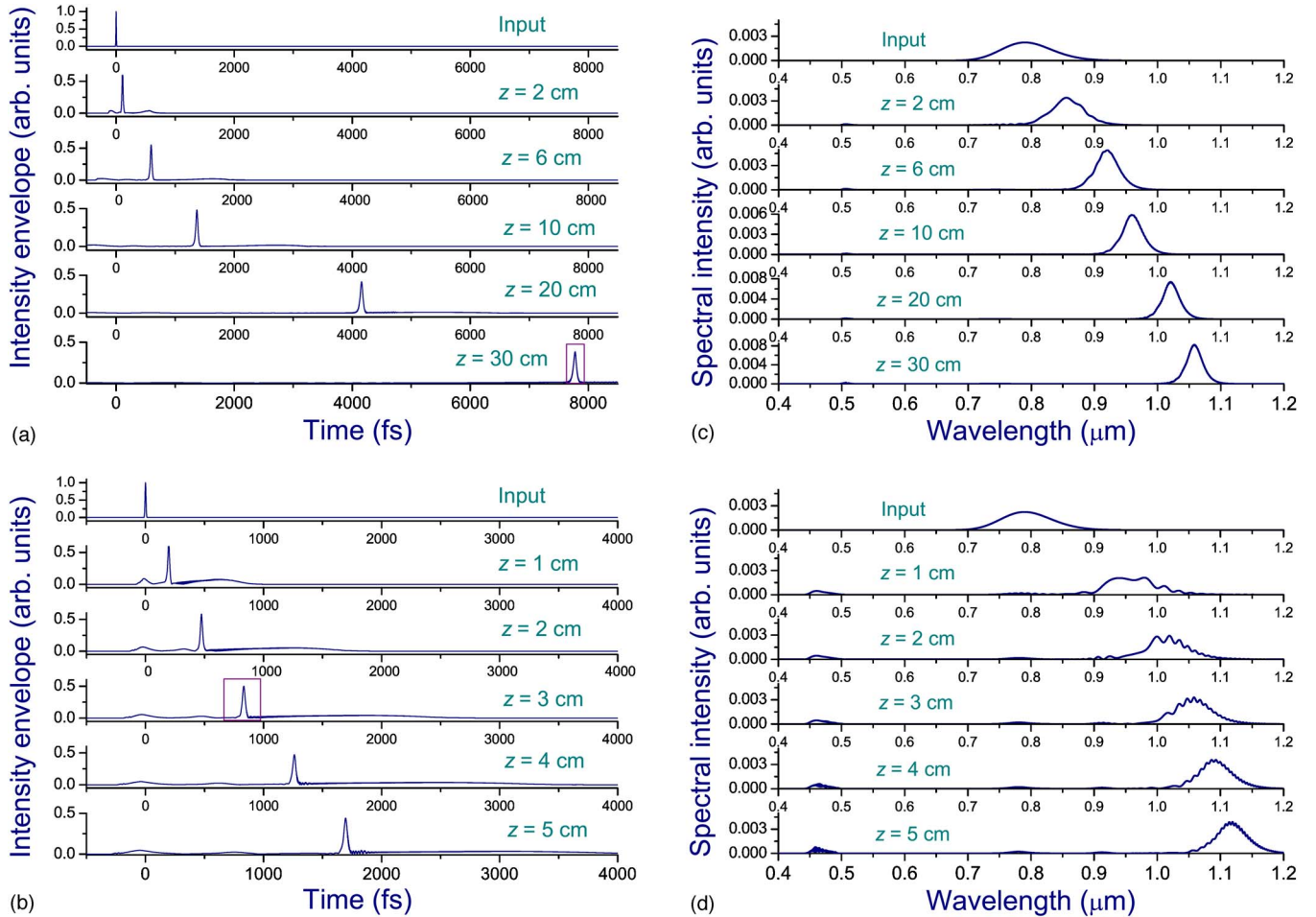
FIG. 2. (Color online) Temporal (a) and (b) and spectral (c) and (d) evolution of laser pulses with an initial energy of (a) and (c) 0.15 nJ and (b) and (d) 0.5 nJ and an initial pulse width of 6 fs in a PCF with a dispersion profile shown by curve 1 in Fig. 1. The input pulses are assumed to be transform-limited.
