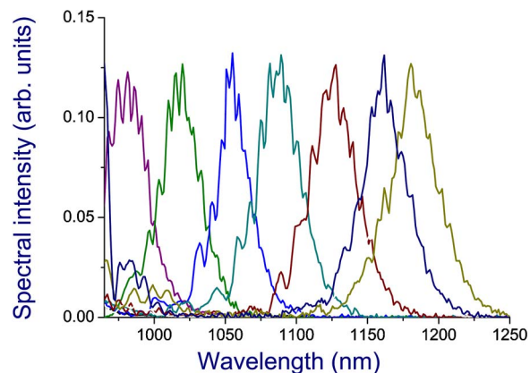
FIG. 10. (Color online) Experimentally measured redshifted output of the NL-PM-750 fiber tuned from 970 to 1170 nm by varying the input energy in the fundamental mode of the PCF.
