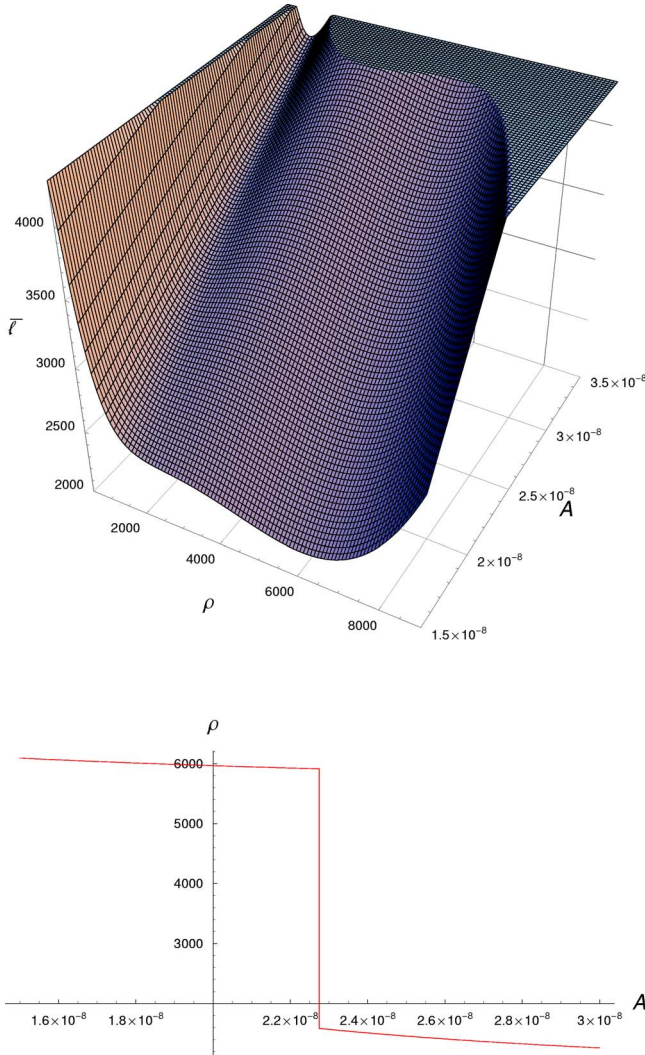
FIG. 4. (Color online) Top: Landscape of the average shortest path length \bar{\ell} (vertical axis) as a function of the cubic cost-function parameter A and the average number of connections to a global hub \rho . Bottom: The value of \rho corresponding to a global minima in \bar{\ell} , as a function of the cubic cost parameter A .
