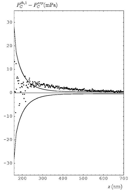
FIG. 3. Differences of theoretical and experimental parallel plate Casimir pressures vs separation obtained from the improved dynamic measurement of Ref. [15] after all separation distances have been decreased by 1 nm to take into account the hypothetical systematic error suggested by Ref. [16]. The theoretical values for P_C^{th,1} are calculated as in Refs. [1–5]. Solid lines represent the 95% confidence interval.
