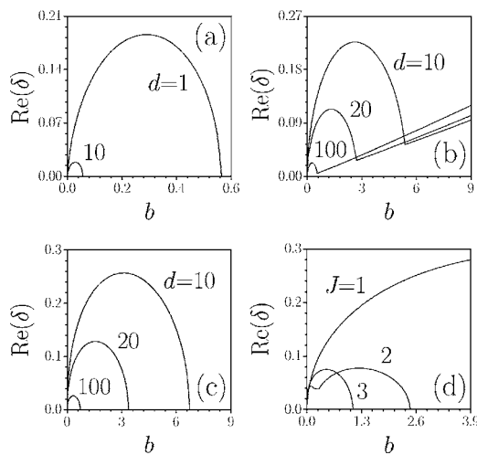
FIG. 3. The real part of the perturbation growth rate vs the propagation constant of the unperturbed soliton. (a) S=0, J=0 , for d=1 and d=10 ; (b) S=1, J=1 ; (c) S=1, J=2 ; (d) S=2, d=20 . In (b) and (c), values of d , and in (d), values of J are indicated near the curves.
