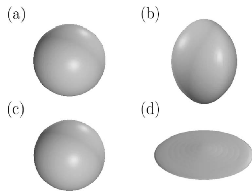
FIG. 5. Self-trapping of a fundamental soliton, for d=1 : (a) and (c) the initial Gaussian pulse with energy E_0=54 ; (b) and (d) the soliton at \xi=60 .
