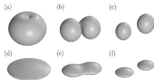
FIG. 6. Splitting of an unstable S=1 soliton with d=100 and b=0.05 . (a) and (d) \xi=0 , (b) and (e) \xi=1400 , and (c) and (f) \xi=1600 .
