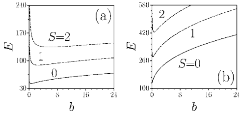
FIG. 1. Energy E vs propagation constant b for soliton families with different vorticities, S=0, 1 , and 2 (numbers labeling the curves), at different values of the range of nonlocality of nonlinear response \sqrt{d} : (a) d=1 , (b) d=10 . Full and dashed lines show stable and unstable solitons.
