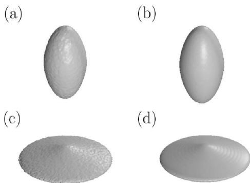
FIG. 4. Isosurface plots illustrating the stability of a fundamental soliton corresponding to d=10, b=1 , and E=178 . (a) and (c) The initially perturbed soliton, at \xi=0 ; (b) and (d) the self-cleaned one at \xi=360 . Here and in Figs. 5 and 6, the upper and lower rows show |q|^2 and n , respectively.
