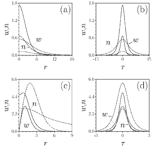
FIG. 2. Cross-section shapes of typical S=0 and S=1 solitons in the transverse ( r ) and temporal ( \tau ) directions. (a) and (b) S=0 , d=10 , E=140 ; full and dashed lines correspond to stable and unstable solitons, with b=0.15 and b=0.021 , respectively. (c) and (d) S=1 , b=1 ; solid and dashed lines correspond to d=1 and d=100 , respectively (due to the scaling invariance, the latter is tantamount to d=1 and b=100 ).
