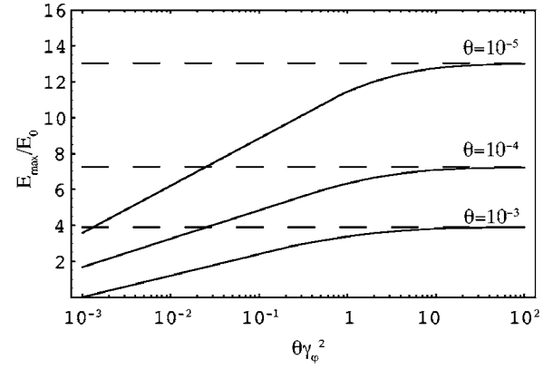
FIG. 1. Maximum plasma wave electric field \hat{E}_{\max} = E_{\max}/E_0 [Eq. (11)] vs \theta\gamma_\phi^2 for initial temperatures \theta=10^{-3} , \theta=10^{-4} , and \theta=10^{-5} , with \gamma_\perp=1 . Dashed lines are the ultrahigh phase velocity result \beta_\phi=1 [Eq. (13)].
