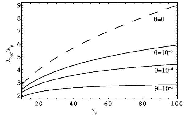
FIG. 2. Normalized nonlinear plasma wavelength \lambda_{\text{osc}}/\lambda_p at the maximum plasma wave amplitude vs \gamma_\phi for initial temperatures \theta=10^{-3} , \theta=10^{-4} , and \theta=10^{-5} , with \gamma_\perp=1 . The dashed line is the cold limit \theta=0 .
