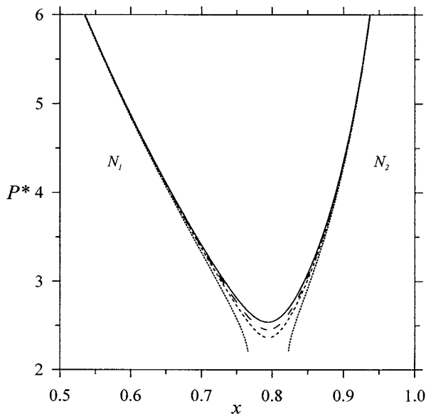
FIG. 8. The effect of the aspect ratio on the pressure-composition ( P^* - x ) representation of the nematic-nematic lower critical point of the system of thick (component 1) and thin (component 2) rods using the Onsager trial function with inclusion of higher order terms in 1/\alpha_i [Eq. (36)] for diameter ratios d = D_2/D_1 = 0.222 : k = 1000 (continuous curve), 200 (long dashed curve), 150 (short dashed curve), and 100 (dotted curve). The mole fraction is that of the thin rods ( x = x_2 ).
