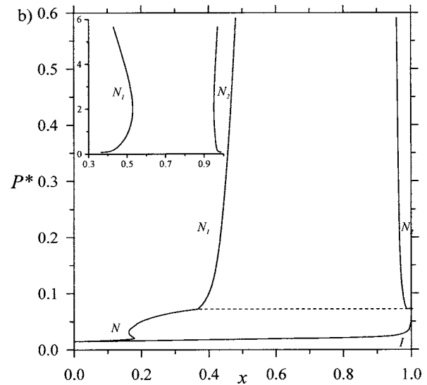
FIG. 9. Reduced pressure-composition ( P^* - x ) representations of the phase diagram of the system of thick (component 1) and thin (component 2) rods obtained with the Onsager theory at aspect ratio k = L/D_1 = 1000 : for diameter ratios (a) d = D_2/D_1 = 0.222 and (b) d = 0.2 . The resulting phase diagrams are obtained by Onsager trial function method. The continuous curves correspond to the phase boundaries of the isotropic-nematic transition and nematic-nematic demixing transitions, while the dashed line represents the isotropic-nematic-nematic three-phase lines. The insets show the nematic-nematic phase boundary in the region of higher pressures. The diamonds show the location of the nematic-nematic critical point, while the labels I and N denote isotropic and nematic phases, respectively. The mole fraction is that of the thin rods ( x = x_2 ).
