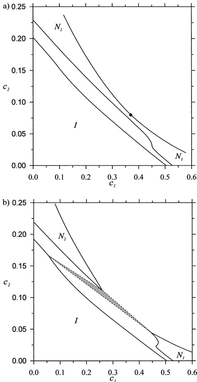
FIG. 15. Composition-composition ( c_2-c_1 ) representations of the phase diagram of the system of thick (component 1) and thin (component 2) rods obtained with the Parsons-Lee theory at aspect ratio k=L/D_1=4 and diameter ratios of d=0.286 (a) and d=0.270 (b). The continuous curves correspond to the phase boundaries of the isotropic-nematic and nematic-nematic phase transitions. The three-phase region is indicated by the gray triangle in figure (b). The diamonds show the location of the nematic-nematic critical point, while the labels I and N denote isotropic and nematic phases, respectively.
