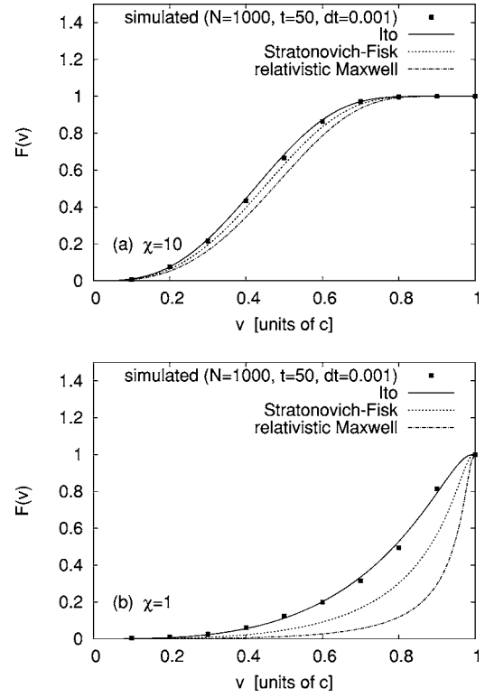
FIG. 1. These diagrams depict a comparison among the numerical Ito prescription and the three analytical results for the corresponding stationary cumulative distribution function F(v) in the laboratory frame \Sigma_0 . (a) In the nonrelativistic limit \chi \gg 1 the stationary solutions of the three different FPE's are nearly indistinguishable. (b) In the strong relativistic limit case \chi \leq 1 , however, the stationary solutions exhibit deviations from each other. Because our simulations are based on an Ito discretization scheme, the numerical data points do agree with the Ito solution (solid line).
