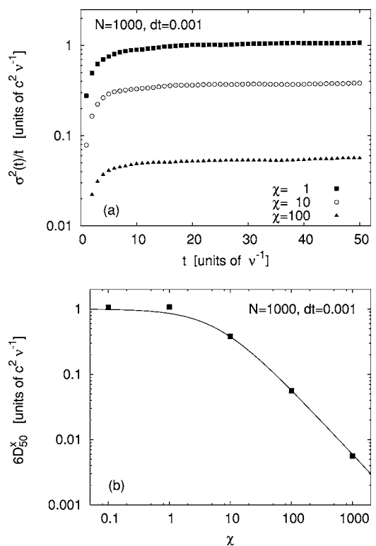
FIG. 3. (a) Mean-square displacement, divided by elapsed time t , as numerically calculated for different \chi values in the laboratory frame \Sigma_0 (rest frame of the heat bath). As evident from this diagram, for the relativistic Brownian motion the related asymptotic mean-square displacement grows linearly with t . (b) The coordinate-space diffusion constant D_{50}^x(\chi) was numerically determined at time t=50\nu^{-1} . The solid line corresponds to the empirical fitting formula D^x(\chi) = c^2\nu^{-1}(\chi+6)^{-1} , which reduces to the classical nonrelativistic result D^x \approx c^2\nu^{-1}(\nu\chi) = kT/(m\nu) for \chi \gg 6 .
