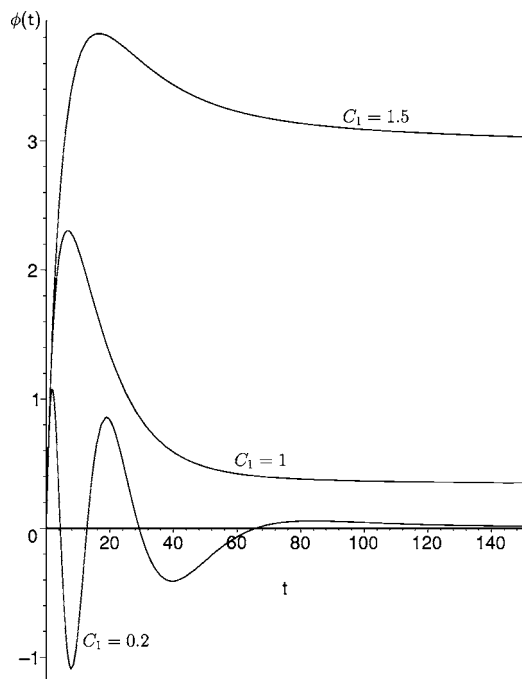
FIG. 1. Influence of the stretch rate C_1 in the X -direction on the shearing motion solutions for a Blatz-Ko material (foamed, polyurethane elastomer).
