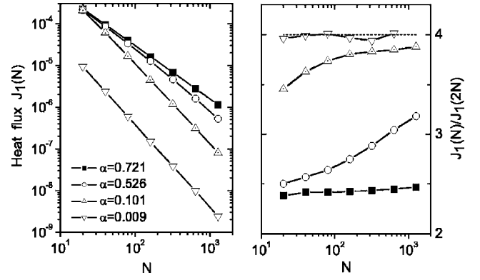
FIG. 3. The heat flux of a single particle versus system size ( N=20, 40, 80, 160, 320, 640 , and 1280 ) with the divergence exponent of heat conductivity \alpha=0.721, 0.526, 0.101 , and 0.009 for four typical cases, respectively (left panel). The ratio of heat flux is J_1(N)/J_1(2N) for different system sizes (right panel).
