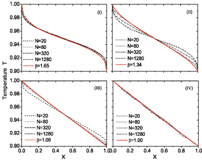
FIG. 6. (Color online) Numerical results of temperature profiles for T_L=1.0 , T_R=0.9 , and sizes N=20 (dash), 80 (dot), 320 (dash dot), and 1280 (dash dot dot), respectively. The four panels refer to (I) R=0 , h=1.0 ; (II) R=0.001 , h=1.0 ; (III) R=0.848\ 528 , h=1.0 ; and (IV) R=0.84\ 528 , h=0.27 . The solid lines correspond to the best fits for the numerical temperature profile at N=1280 with Eq. (8), giving the analytical values \beta with 1.65, 1.34, 1.06, and 1.00 for the above four cases, respectively.
