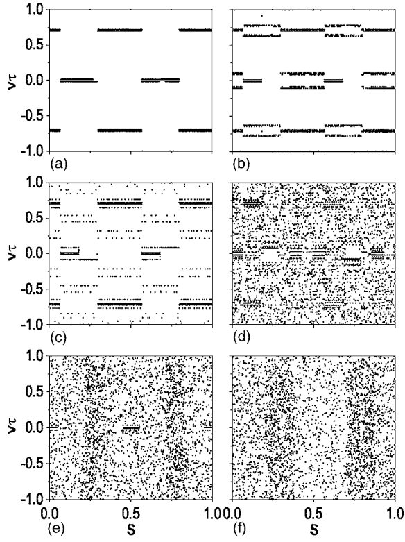
FIG. 2. Poincaré surface-of-section of the billiard problem. The billiard starts with an incident angle 0.8 and unit velocity. (a) R=0 , h=1.0 ; (b) R=0.001 , h=1.0 ; (c) R=0.015 , h=1.0 ; (d) R=0.1 , h=1.0 ; (e) R=0.848\ 528 , h=1.0 ; and (f) R=0.848\ 528 , h=0.27 .
