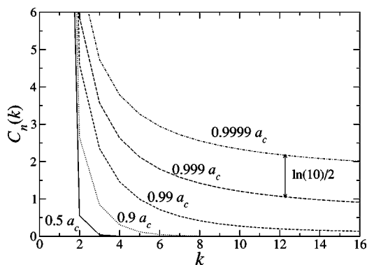
FIG. 6. Multiscale complexity for the one-dimensional spin chain with nearest-neighbor interactions, for different interaction strengths at n=16 .
