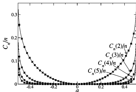
FIG. 5. Multiscale complexities for the multispin chain, normalized by the number of spins, n , for n=16 (lines), n=25 (squares), and n=32 (crosses).
