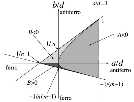
FIG. 9. Phase diagram for a block matrix with m groups of n spins each. Relevant variables are the ratios between near- and far-neighbor interactions and self-interaction. Shading indicates the sign of covariances A and B .
