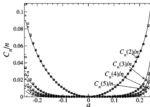
FIG. 7. Multiscale complexities for the square lattice with nearest-neighbor interactions, normalized by the number of spins, n=L \times L , for L=5 (lines), L=6 (squares), and L=7 (crosses).
