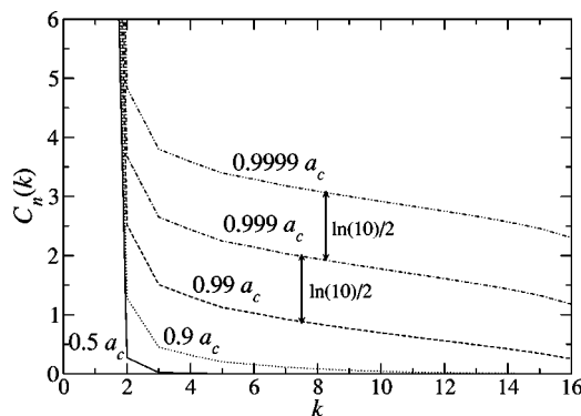
FIG. 8. Multiscale complexity for the square lattice with nearest-neighbor interactions, for different interaction strengths at L=4 .
