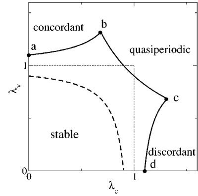
FIG. 5. Stability boundaries from the map analysis for positive coupling C=0.1 with concordant alternans along the dashed line, and negative coupling C=-0.1 (solid line), with concordant alternans, discordant alternans, and quasiperiodicity along the segments a-b, c-d, and b-c, respectively.
