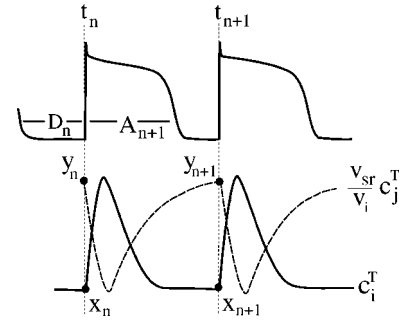
FIG. 4. Definition of map variables.
