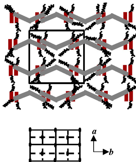
FIG. 16. Schematic representation of the molecular arrangement in the B_1' phase of M30 ( a=56.5 \text{ \AA} and b=64 \text{ \AA} ).
