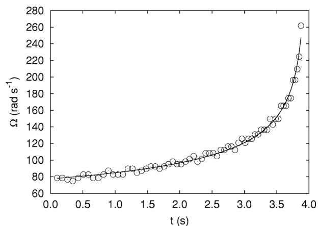
FIG. 9. Temporal evolution of the precession rate \Omega for the aluminum disk case on the aluminum surface. A fit using Eq. (3) is also illustrated.
