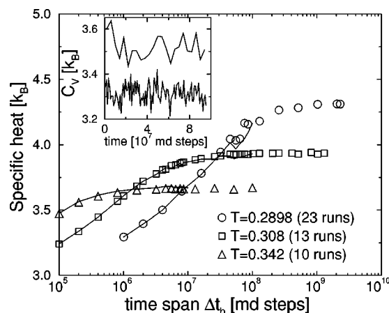
FIG. 2. Block averaged specific heat vs time span \Delta t_b for 512 particles at T=0.289\,855 , 0.308\,642 , and 0.342\,4658 . Solid lines are the result of block averaging each run and then averaging over the number of runs shown. Open symbols are the result of stringing runs together and then block averaging. The shape of the symbols indicates the temperature as given in the legend. Inset: Block averaged specific heat vs time for 512 particles at T=0.289\,855 . The lower curve corresponds to \Delta t_b=10^6 MD steps, and the upper to \Delta t_b=4 \times 10^6 MD steps. The time is the time (in units of 10^7 MD steps) in the middle of each block. The data at T=0.289\,855 is averaged over 23 runs. Parameters for both figures are the same as in Fig. 1.
