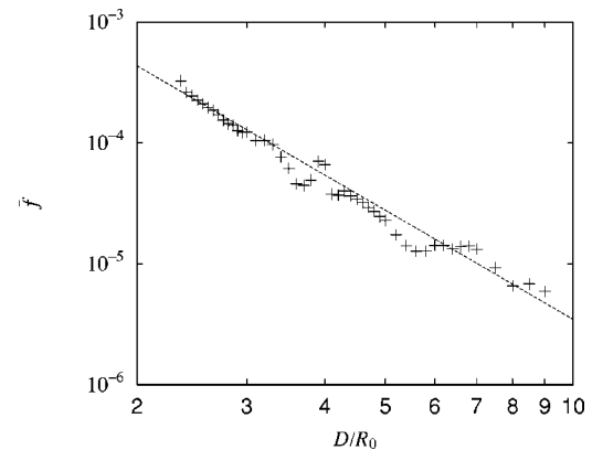
FIG. 8. Log-log plot of the dimensionless force \bar{f} as a function of D in the case of the “antiparallel-dipole” configuration. The dashed line corresponds to 0.003\,45(D/R_0)^{-3} .
