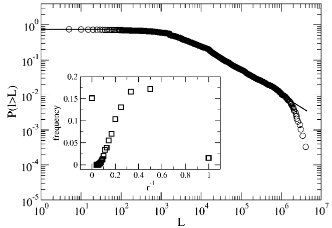
FIG. 2. The probability that a substation has more than L transmission paths passing through it. The continuous curve has the generalized power law form (2). Inset: histogram of the length of the shortest alternative path r between the end points of an edge. In order to be able to include edges with no alternative path, the abscissa is inverted.
