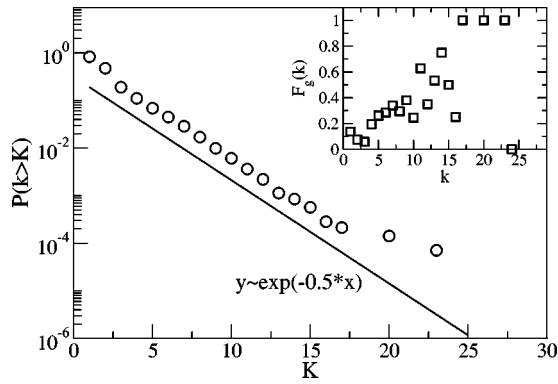
FIG. 1. The probability that a substation has more than K transmission lines. The straight line represents the exponential function (1). Inset: the fraction F_g(k) of generating substations among substations with degree k .
