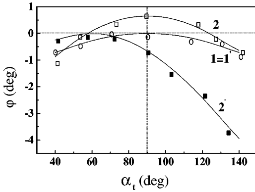
FIG. 3. Analyzer angle vs sample rotation curves for films of polymer P1 before (curves 1, 1') and after (curves 2, 2') UV irradiation ( \alpha_{uv}=45^\circ , I=12 mW/cm 2 , and t=10 min). Curves 1, 2 and 1', 2' correspond to vertical and horizontal orientations, respectively. According to the model used, n_x=n_y=n^o < n_z=n^e , (n^e-n^o)d=5 nm, \theta_a=90^\circ (before irradiation) and (n^e-n^o)d=30 nm, \theta_a=71^\circ (after irradiation).
