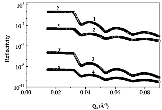
FIG. 7. Specular reflectivity scans for a film of P1, before and after irradiation with nonpolarized UV light ( \alpha_{UV}=90^\circ , I=12 \text{ mW/cm}^2 and t=10 \text{ min} ). The scans are presented for x and y orientations of the sample. Fits yield \sigma=19 \pm 1 \text{ \AA} (nonirradiated film) and \sigma=24 \pm 1 \text{ \AA} (irradiated film).
