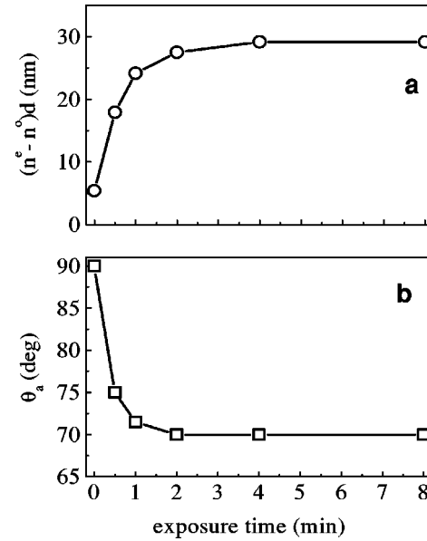
FIG. 4. Phase retardation (a) and tilt angle of azochromophores (b) in P1 film, as functions of irradiation time. Irradiation is performed at \alpha_{uv}=45^\circ , I=12 mW/cm 2 .
