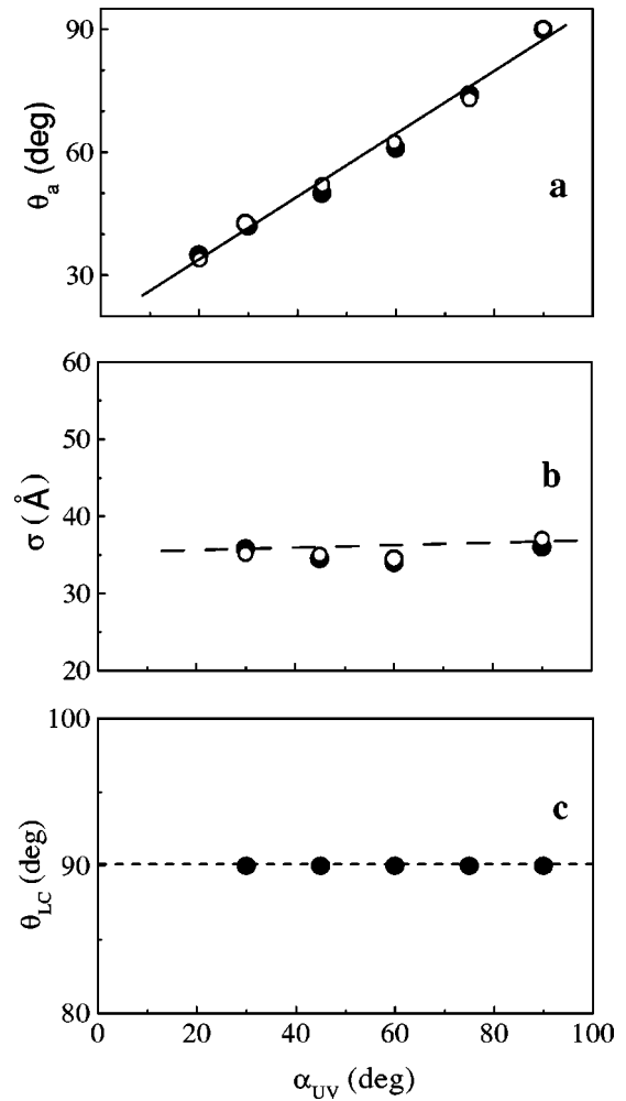
FIG. 6. (a) Azochromophore tilt angle, (b) surface roughness in the x and y directions of the film, and (c) LC pretilt angle for LC 5CB and E7 as functions of the angle of incidence of UV light. The irradiation parameters are I=12 \text{ mW/cm}^2 and t=10 \text{ min} .
