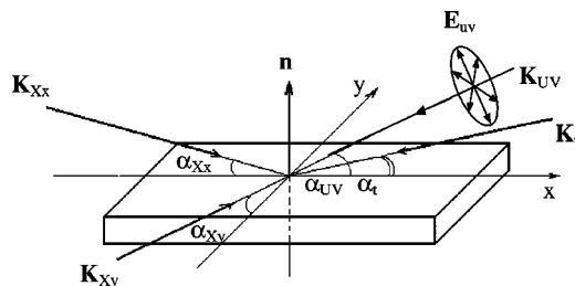
FIG. 2. Sample orientation with respect to the UV beam with wave vector \mathbf{K}_{\text{UV}} , probe beam with wave vector \mathbf{K}_t , and incident x-ray beam with wave vector \mathbf{K}_{xi} ( i=x,y ). n is surface normal. x and y axes lie in substrates plane.
