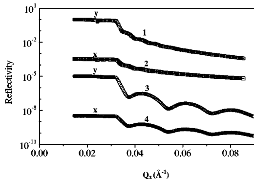
FIG. 8. Specular reflectivity scans for the film of polymer P2 before and after irradiation with nonpolarized UV light ( \alpha_{uv} = 90^\circ , I = 12 \text{ mW/cm}^2 and t = 10 \text{ min} ). The scans are presented for x and y orientations of the sample. Fits give \sigma = 55 \pm 1 \text{ \AA} (nonirradiated film), \sigma = 36 \pm 1 \text{ \AA} (irradiated film).
