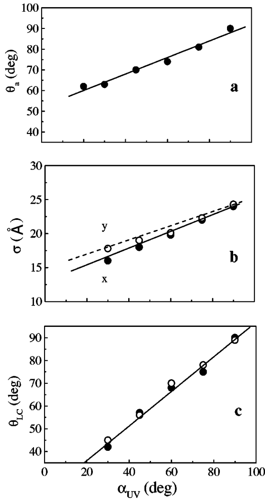
FIG. 5. Azochromophore tilt angle (a), surface roughness (b), and LC pretilt angle (c) as functions of the angle of incidence of UV light for P1 films. The irradiation parameters are I=12 \text{ mW/cm}^2 , t=10 \text{ min} . In (b) data marked with x and y correspond to roughness in the x and y directions of the film. In (c) solid and open circles correspond to LC 5CB and LC ZL14801, respectively.
