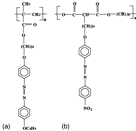
FIG. 1. Structural formulas of (a) polymer P1 and (b) polymer P2 .
