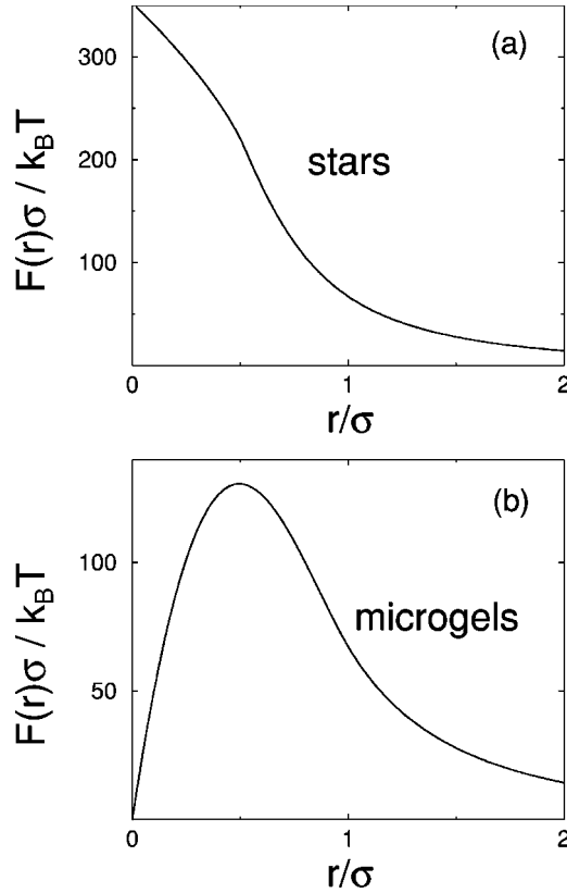
FIG. 4. Effective electrostatic forces between pairs of polyelectrolyte stars (a) and microgels (b), corresponding to the interaction potentials in Fig. 3. Parameters are the same as in Fig. 1.
