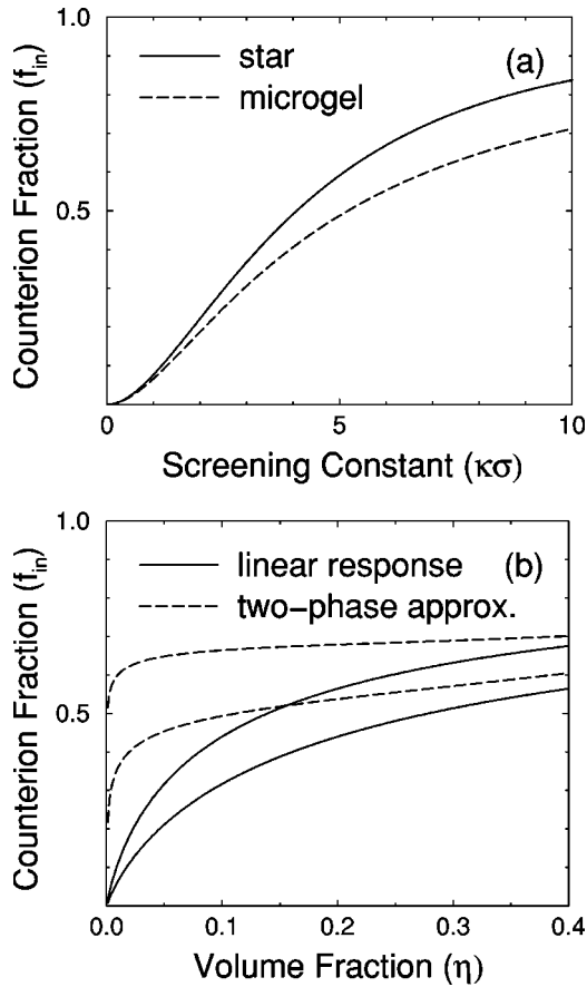
FIG. 2. (a) Fractions of counterions [from Eqs. (24) and (38)] inside polyelectrolyte star and microgel macroions vs Debye screening constant \kappa . (b) Fraction of counterions inside a uniformly charged spherical macroion vs effective macroion volume fraction as predicted by linear response theory (solid curves) and by the two-phase approximation of Oosawa [1] (dashed curves). For each case, the bottom curve corresponds to Z\lambda_B/a = 8 and the top curve to Z\lambda_B/a = 16 .
