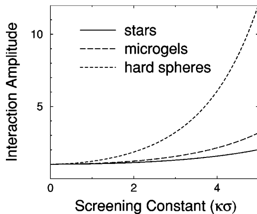
FIG. 5. Macroion-size-dependent amplitude of Yukawa effective electrostatic interactions [Eqs. (28), (29), and (41)] between pairs of nonoverlapping stars, microgels, and hard spheres vs Debye screening constant, normalized to unity at \kappa\sigma = 0 .
