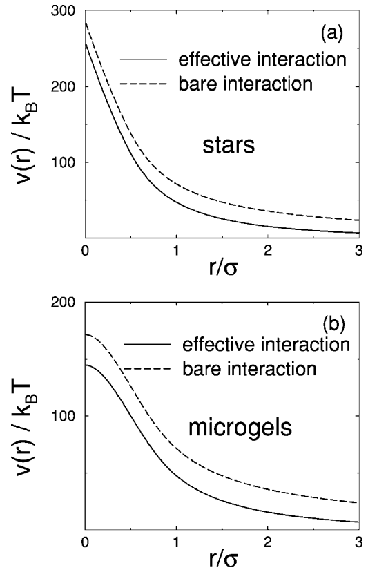
FIG. 3. Electrostatic interactions [from Eqs. (28) and (41)] between pairs of polyelectrolyte stars (a) and microgels (b). Dashed curves: bare interaction. Solid curves: effective (bare + induced) interaction. Parameters are the same as in Fig. 1. Beyond overlap ( r/\sigma > 1 ), the interaction is Yukawa in form. For overlapping macroions ( r/\sigma < 1 ), the soft repulsion remains finite at complete overlap ( r = 0 ).
