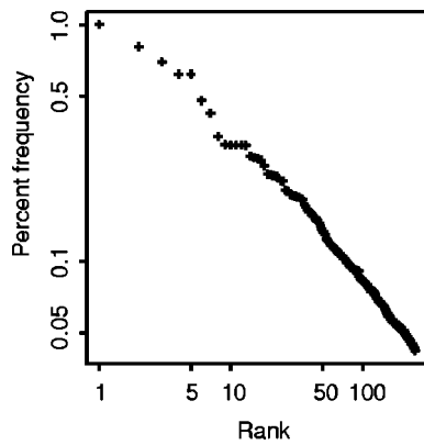
FIG. 5. Family names in the 1990 US Census: logarithmic plot of rank against frequency for the most common 250 names, with the upper left point for the most common name.
