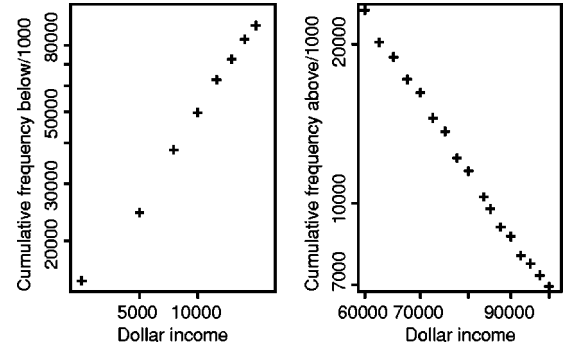
FIG. 2. Distribution of the total money income of 216 \times 10^6 people in USA in 2000. The left and right panels show (on logarithmic axes) the cumulative frequency distributions (binned) in the lower and upper tails, respectively, suggesting power laws (unbinned income data are not available).
