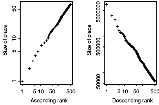
FIG. 1. Distribution of the sizes of 19 399 places in the USA in 1999. Logarithmic rank-size plots of the smallest 500 places (left panel) and the largest 500 places (right panel) suggest power-law behavior in both tails of the distribution.
