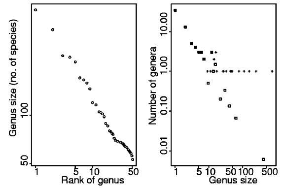
FIG. 4. Logarithmic plots of the observed sizes of 1829 genera of North American vascular plants. The left-hand panel is a rank-size plot for the largest 50 genera. The straight-line behavior suggests upper-tail power-law behavior in the genus size distribution. The right-hand panel shows frequency against genus size (crosses) along with a similar plot with binning (boxes), so that each bin contains at least two genera.
