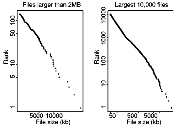
FIG. 3. Logarithmic rank-size plots for the upper tail of the distribution of 734 814 http response sizes at the University of North Carolina at Chapel Hill Main Link [9].
