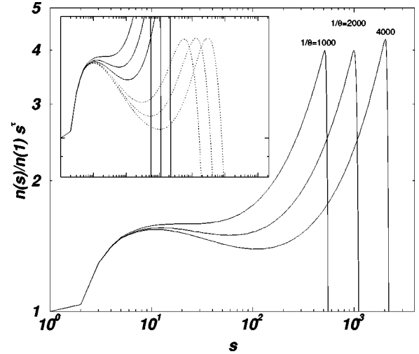
FIG. 8. The rescaled and binned histogram \tilde{n}(s; \theta)s^{7^*} (again \tau^* = 2.10 ), for a modified model, where the largest cluster in the system is removed after each driving step, for 1/\theta = 1000, 2000, 4000 (as indicated) with linear sizes L = 2000, 2000, 4000 . The inset shows the same data on the scale of Fig. 3 for comparison. The data for 1/\theta = 1000, 2000, 4000 of the original model as shown in Fig. 3 are dotted. The peculiar behavior of the different height scaling of the minimum and the maximum is again visible.
