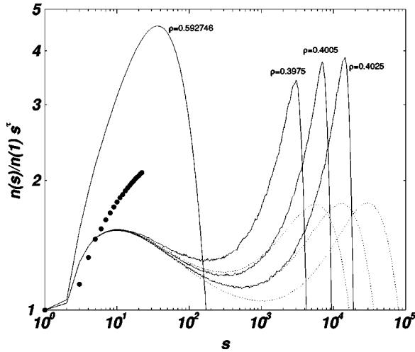
FIG. 9. The rescaled and binned histogram \tilde{n}(s;\rho)s^{\tau^*} (again \tau^*=2.10 ) for a modified model, where the largest cluster in the system is removed in each relaxation step and the corresponding number of trees is filled back into the system afterwards. The three small values of \rho chosen as \rho=0.3975, 0.4005, 0.4025 correspond (up to the last digit) to the values of the tree density for 1/\theta = 1000, 2000, 4000 , respectively, see Table I. The linear size was L = 1000, 2000, 4000 . The corresponding data of the original model are shown dotted. The peculiar behavior of the different height scaling of the minimum and the maximum is again visible (a correct tilt \tau^* would make it even more pronounced), but disappears obviously for \rho = \rho_{\text{perc}} —for these data it is relevant to mention that \tilde{n}(s) was measured after the relaxation. The filled circles show the exact results for the lattice animals [5,17,18] at \rho = \rho_{\text{perc}} .
