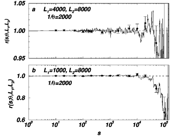
FIG. 1. Ratio r(s; \theta, L_1, L_2) = \tilde{n}(s; \theta, L_1) / \tilde{n}(s; \theta, L_2) with 1/\theta = 2000 for two pairs L_1, L_2 with error bars (standard deviation of 1; the error bars as well as the data shown are exponentially binned). The data are from short runs ( 10^6 updates for statistics). Finite size effects have been considered negligible under the condition that (almost all) error bars for this ratio have covered 1 (marked by a dashed line) in the relevant range. (a) L_1 = 4000 and L_2 = 8000 : almost no finite size effects, the deviation from 1 is probably due to noise. Note the fine scale of the ordinate. (b) L_1 = 1000 and L_2 = 8000 : Systematic, strong finite size effects for s \geq 10^4 . The scale of the ordinate is five times larger than in (a). Data of this quality have been dismissed.
