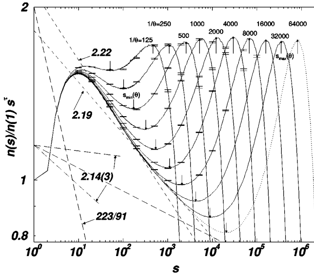
FIG. 3. The rescaled and binned histogram \tilde{n}(s; \theta)s^{\tau^*} , where \tau^* = 2.10 for 1/\theta = 125, 250, 500, \dots, 32\,000, 64\,000 (as indicated) in a double logarithmic plot. The linear size L is chosen according to the bold printed entries in Table I and large enough to ensure absence of finite size effects. The error bars are estimated from shorter runs. The rightmost histogram (dotted in all figures, 1/\theta = 64\,000 ) could not be cross checked by another run (see text). Maxima are marked by arrows pointing upwards, minima are marked by arrows pointing downwards. The dashed lines belong to different exponents, whose values are specified as the sum of the slope in the diagram and \tau^* , i.e., a horizontal line would correspond to an exponent 2.1. The short dashed line represents estimated exponents for different regions of the histogram (2.22 within approximately [20, 200] and 2.19 within [200, 2000] ), the other exponents are from literature, namely, 2.14(3) in Refs. [3,4] and 223/91 \approx 2.45 in Ref. [12]. Since it was impossible to relate these exponents to any property of the data, the exact position of the lines associated with them was chosen arbitrarily.
