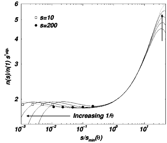
FIG. 5. The rescaled and binned histogram \tilde{n}(s; \theta)s^{\tau_{\text{stp}}} , versus s/s_{\min}(\theta) , where \tau_{\text{stp}} = 2.19 for 1/\theta = 4000, 8000, 16\,000, 32\,000, 64\,000 in a double logarithmic plot. The scales s_{\min}(\theta) by which the histograms have been shifted are slightly different from the minima marked in Fig. 3, to make the collapse as good as possible. The squares and the filled circles mark s = 10 and s = 200 , respectively, for orientation and relation to other figures. The arrows indicate the order of the data in increasing 1/\theta .
