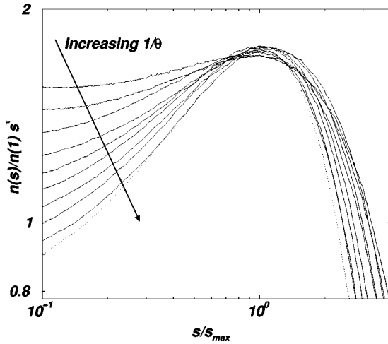
FIG. 4. The rescaled and binned histogram \tilde{n}(s; \theta)s^{\tau^*} , vs s/s_{\max}(\theta) , where \tau^* = 2.10 for 1/\theta = 125, 250, 500, \dots, 32\,000, 64\,000 in a double logarithmic plot. The scales s_{\max}(\theta) by which the histograms have been shifted are the maxima marked in Fig. 3, so that a data collapse would be possible. The arrow indicates the order of the data in increasing 1/\theta .
