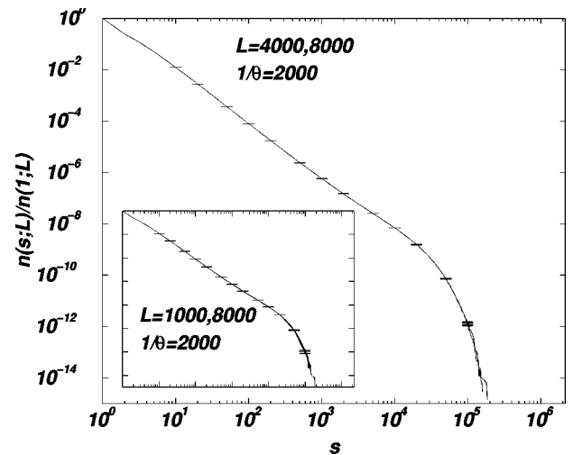
FIG. 2. The binned histogram \tilde{n}(s; \theta, L) for two different values of L and fixed \theta as in Fig. 1(a). In this plot the two histograms are virtually indistinguishable. However, note that the deviations shown on Fig. 1(b) would also hardly be visible in this type of plot, as shown in the inset.
