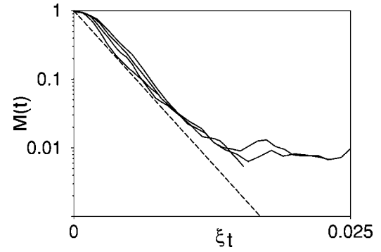
FIG. 4. M(t) as a function of the rescaled time \xi t for k_0=50 and \xi=0.019, 0.038, 0.057, \text{ and } 0.075 . The dotted line gives the decay M(t) = \exp(-\Gamma t/2) .
