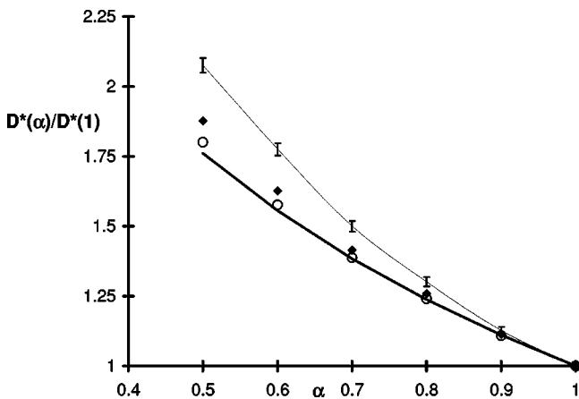
FIG. 9. Diffusion constants for n^*=0.25 as a function of \alpha for 108 atoms, calculated from the Green-Kubo relation (error bars and connecting line), by removing the longest Fourier modes (diamonds), and by using the cell method of computing the local velocity field (circles). All data are normalized to the values determined for \alpha=1 . The heavy line is the prediction from Enskog theory.
