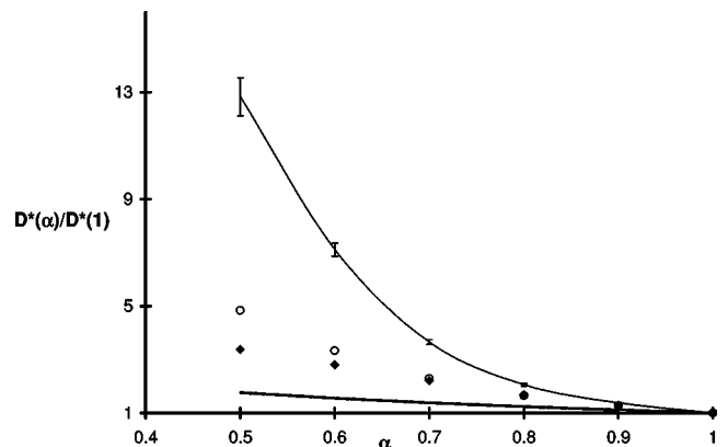
FIG. 11. The same as Fig. 9 for n^*=0.75 .
