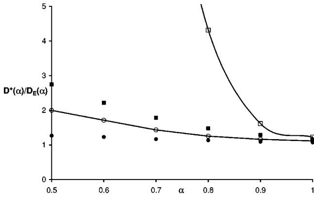
FIG. 8. Diffusion constants for n^*=0.25 (circles) and n^*=0.50 (squares) as a function of \alpha , for 108 atoms (full symbols) and 500 atoms (open symbols). The values are normalized to the \alpha -dependent Enskog prediction. The lines are a guide to the eye.
