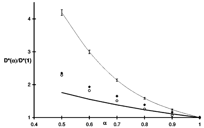
FIG. 10. The same as Fig. 9 for n^*=0.50 .
